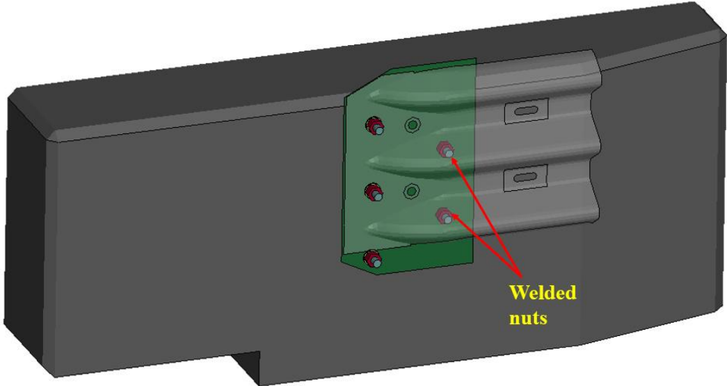
5-Nut Anchorage
