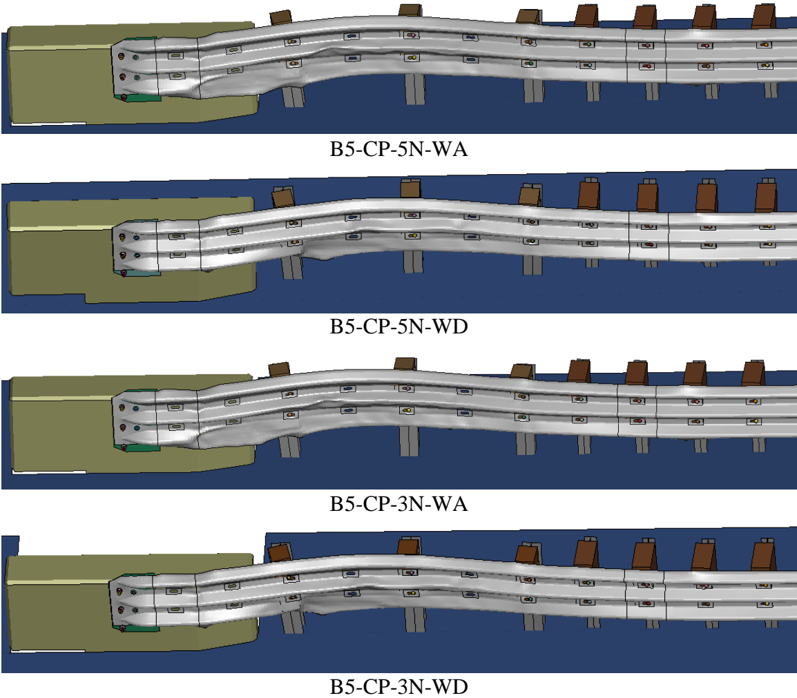
Figure 58. System Damage, Buttress 5
