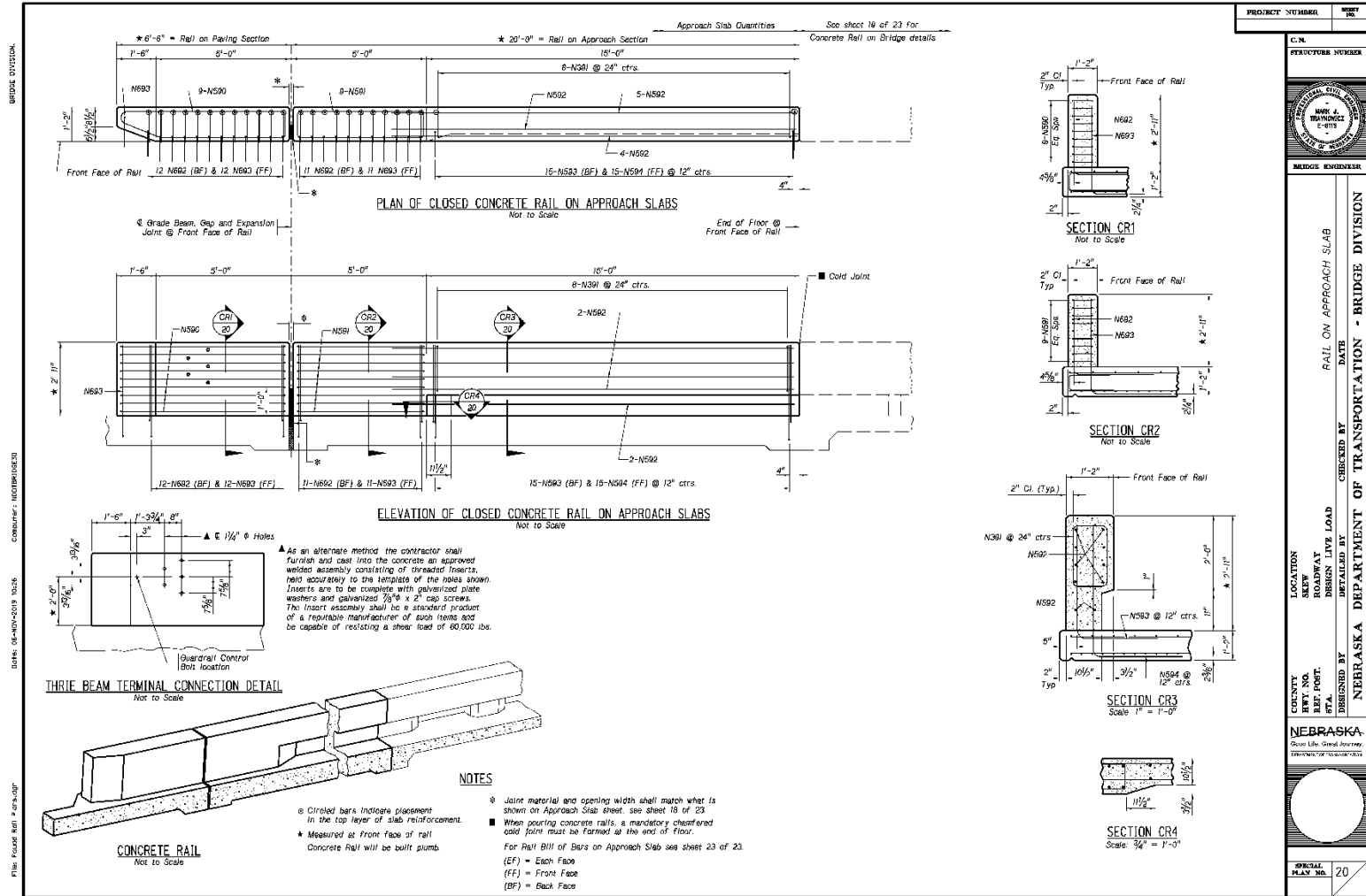
Figure A-7. NDOT Design Details, Buttress 7
