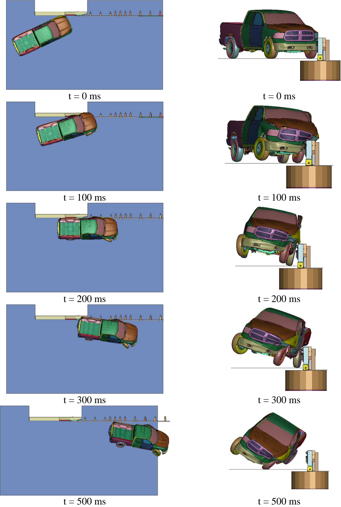
Figure 91. Sequential Images, Simulation No. B2-CP+CF-3N-WA-CFA-REV
