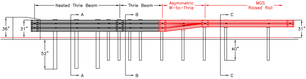
Figure 2. 34-in. Tall AGT After a 3-in. Roadway Overlay [2]
