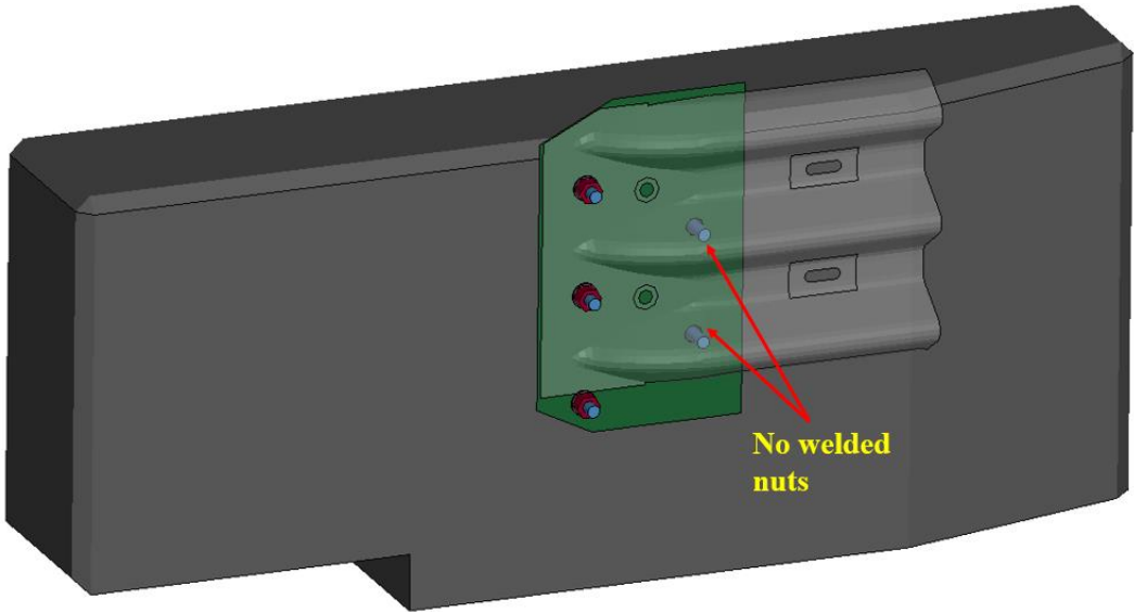
3-Nut Anchorage
