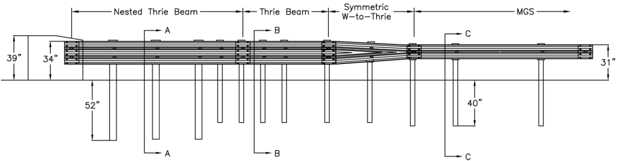
Figure 1. 34-in. Tall AGT Initial Installation, No Overlay [2]
