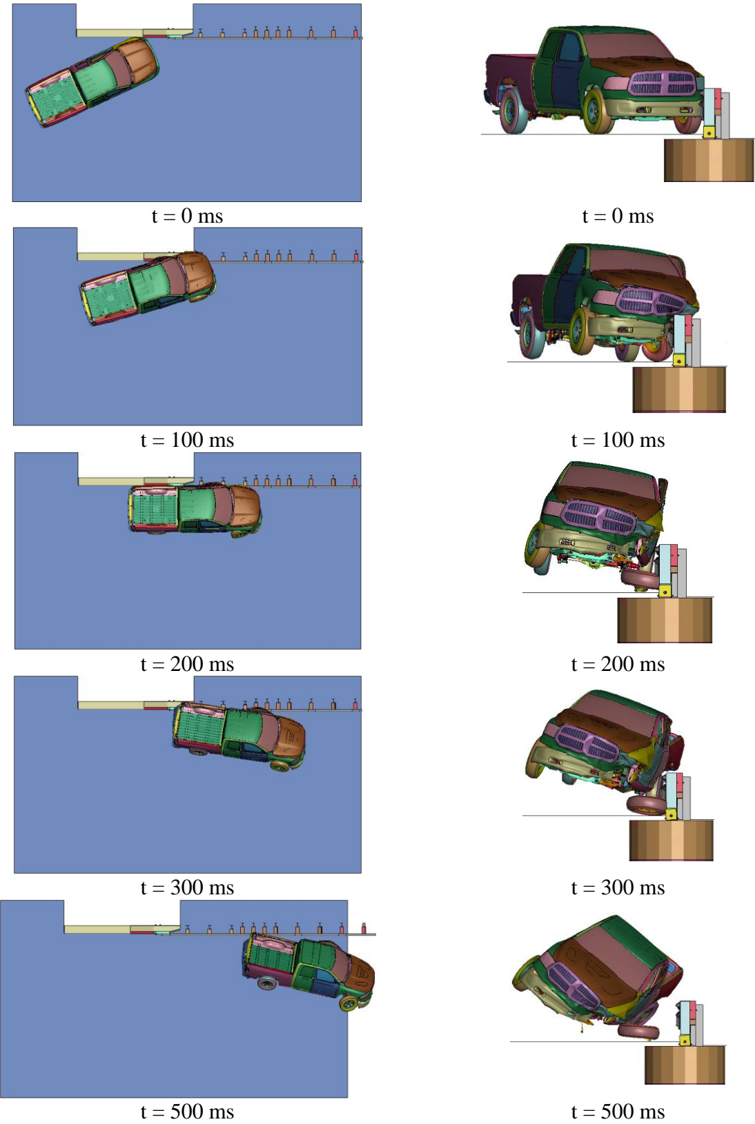
Figure 92. Sequential Images, Simulation No. B2-CP+CF-3N-WD-CFA-REV
