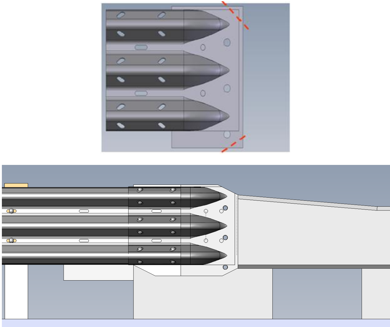
Figure 29. Connector Plate Assembly Corners Cut at 2:1 Slopes for Buttresses 2 and 4
