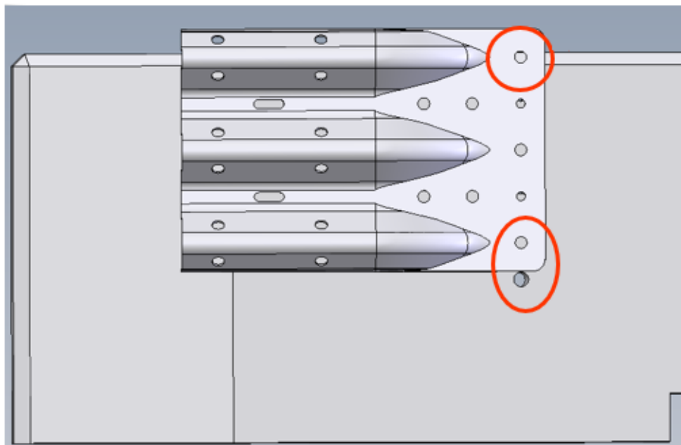
Figure 15. Top Bolt Position with a 32-in. Tall Buttress
