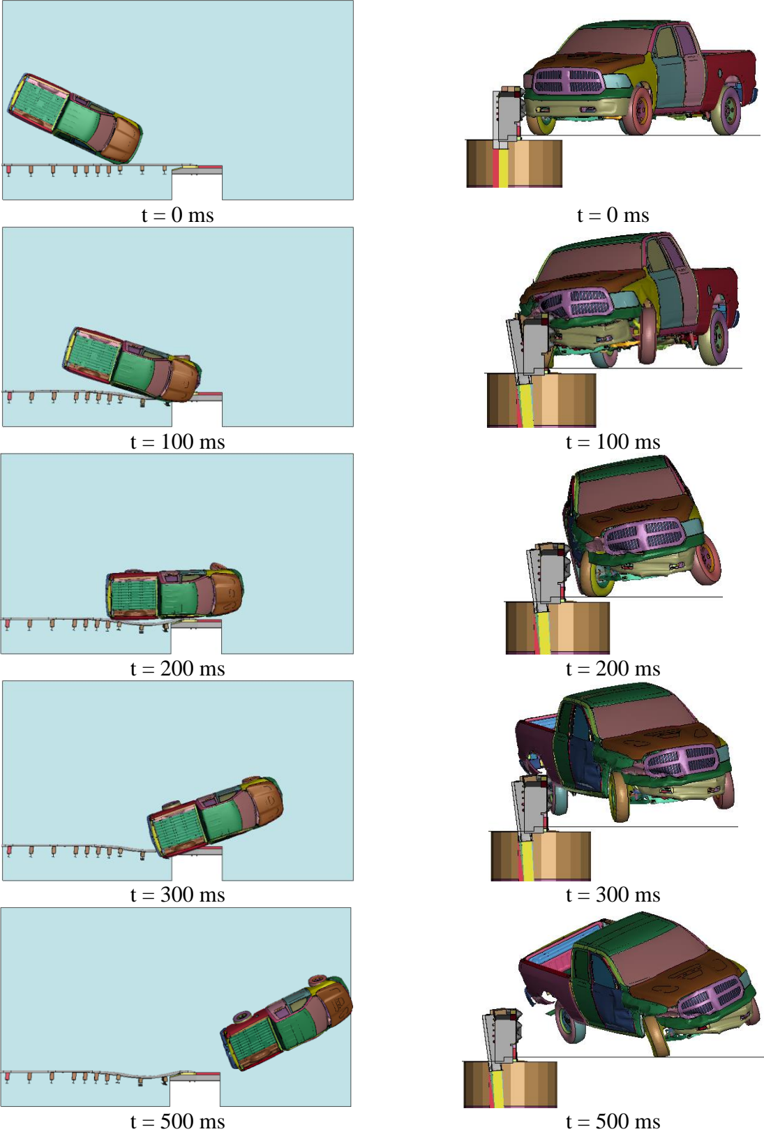
Figure 86. Sequential Images, Simulation No. B2-CP+CF-3N-WA-CFA
