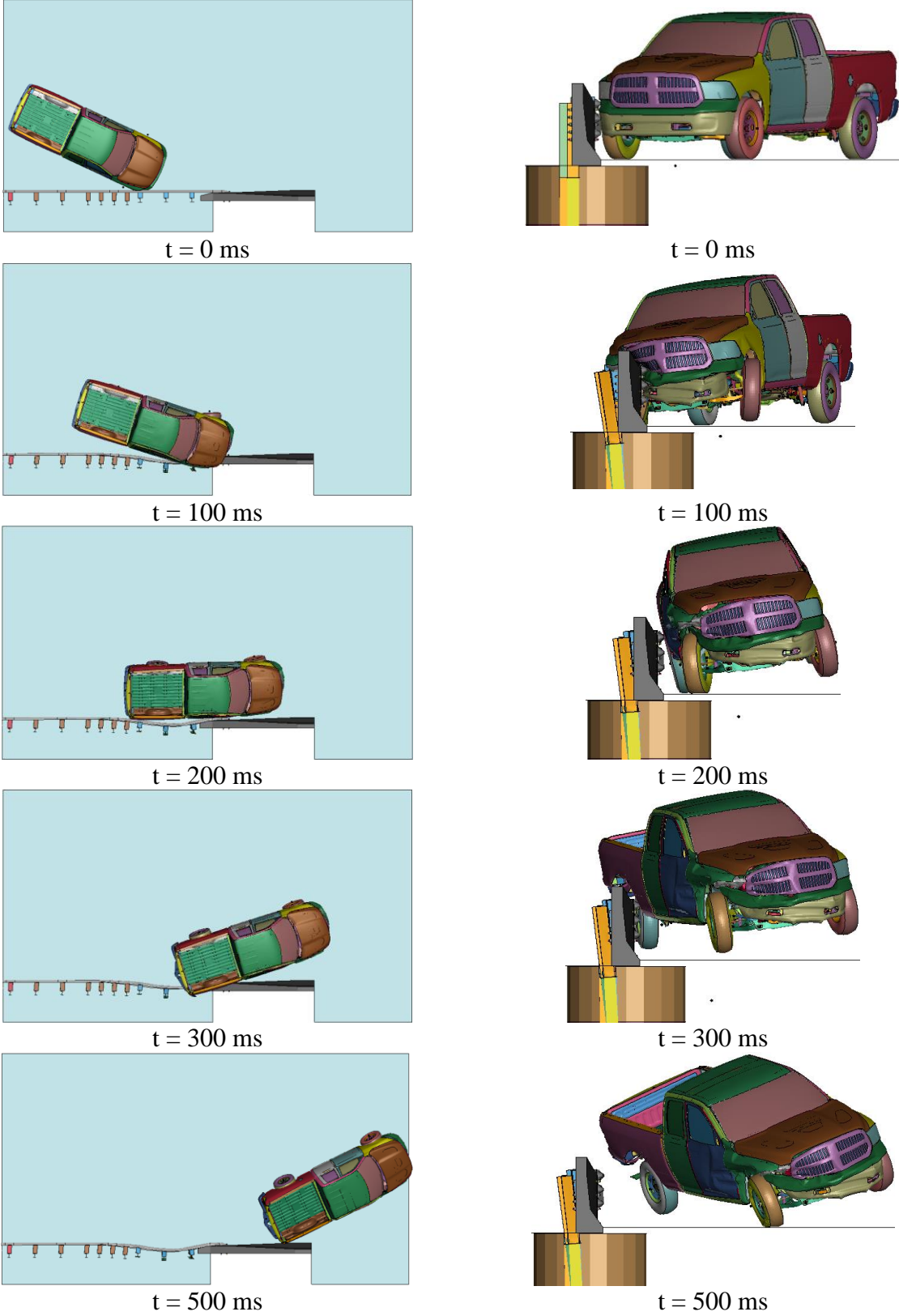
Figure 70. Sequential Images, Simulation No. B8-CP+SA-3N-WA
