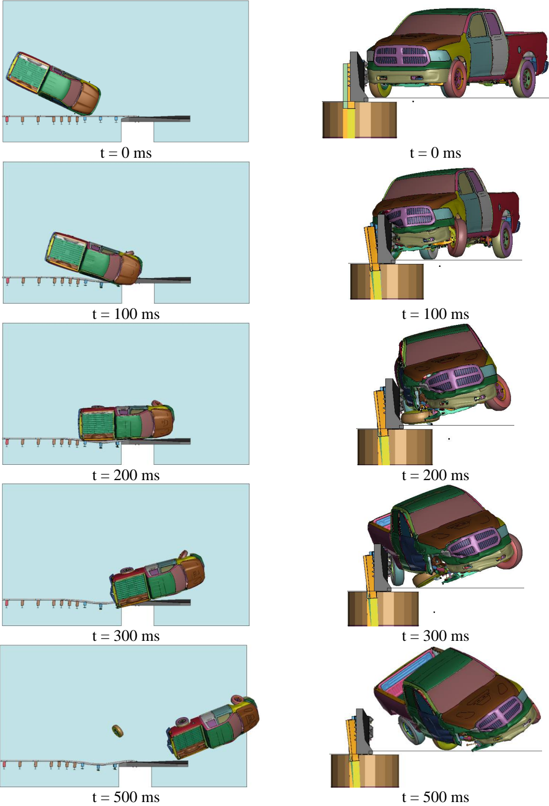
Figure 67. Sequential Images, Simulation No. B8-CP-3N-WD
