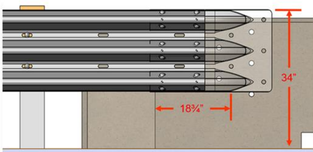
Figure 25. Rail Position on Buttress 5, Adjusted for Height and Unsupported Span Length
