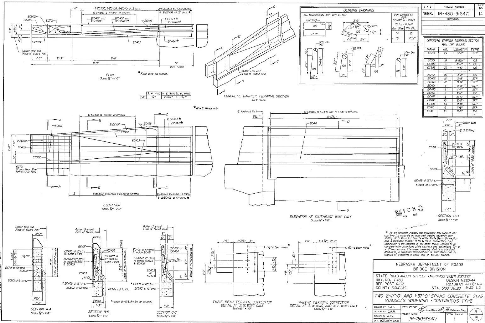
Figure A-8. NDOT Design Details, Buttrass 8
