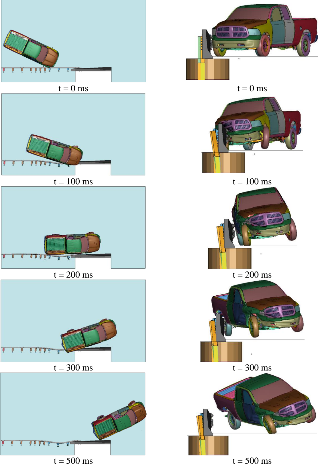
Figure 68. Sequential Images, Simulation No. B8-CP+CF-3N-WA
