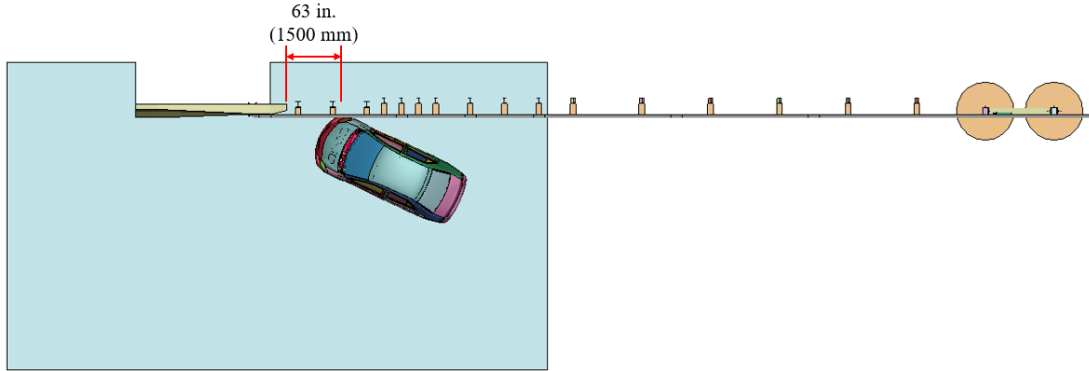
Figure 77. 1100C Vehicle Impact Point
