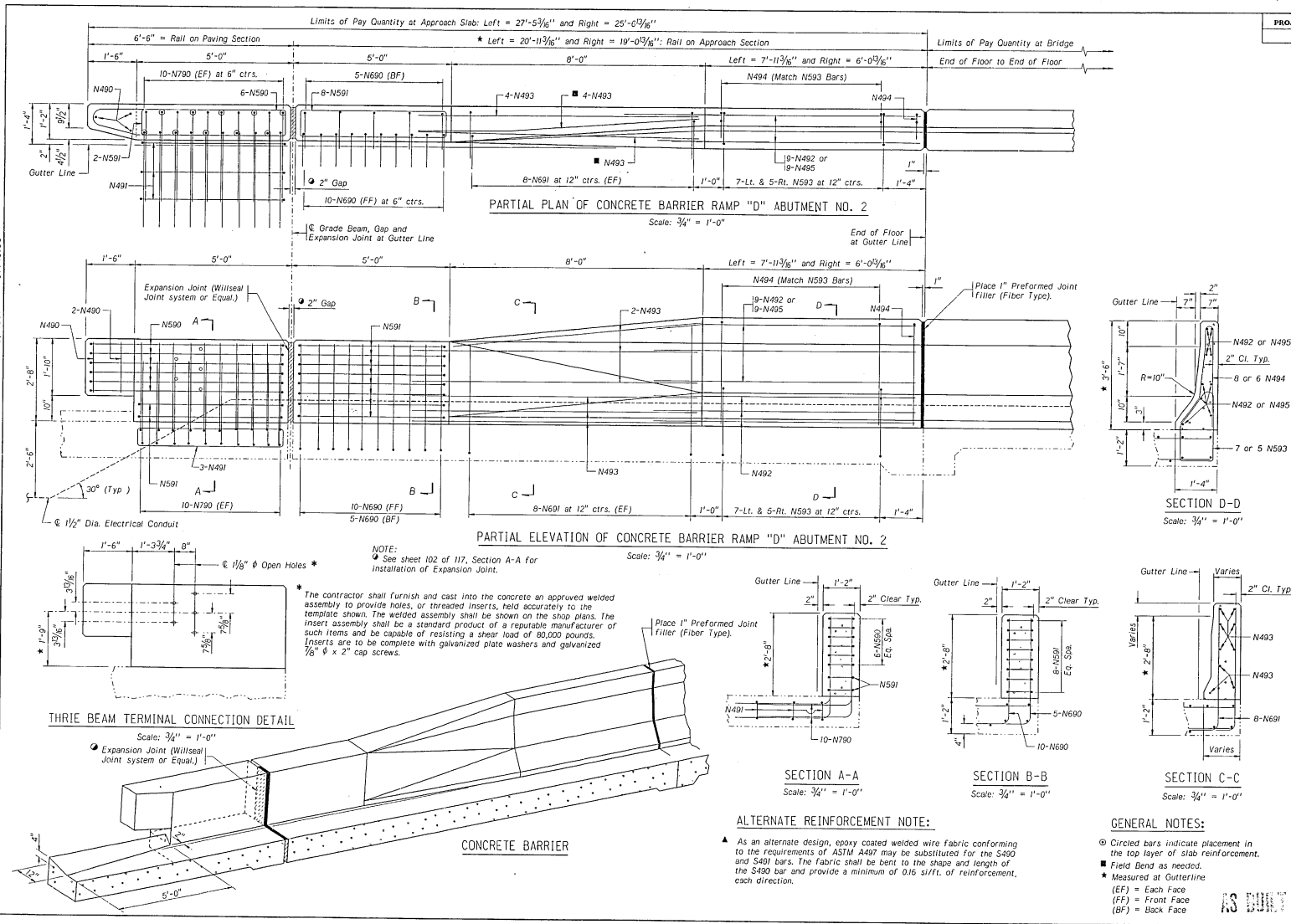
Figure A-10. NDOT Design Details, Buttriss 10
