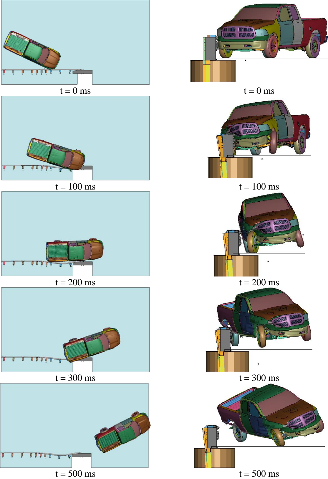
Figure 81. Sequential Images, Simulation No. B10-CP+CF-3N-WA
