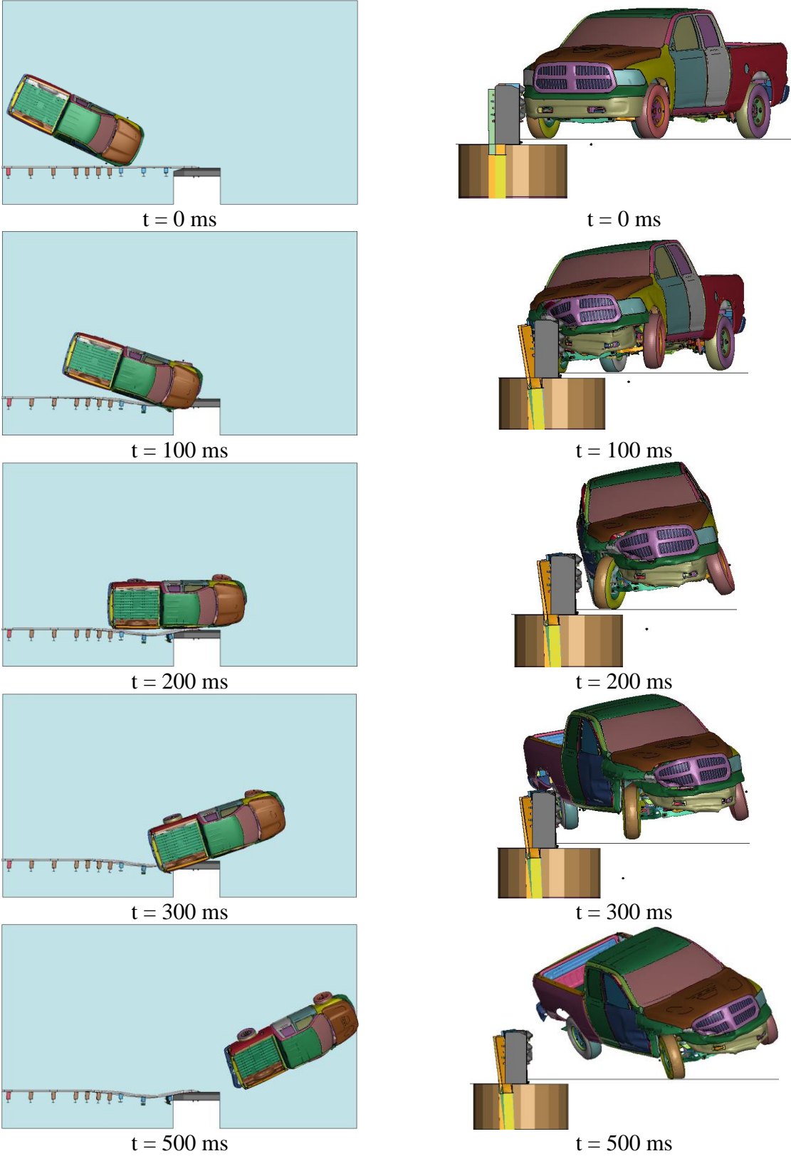
Figure 62. Sequential Images, Simulation No. B6-CP-3N-WA
