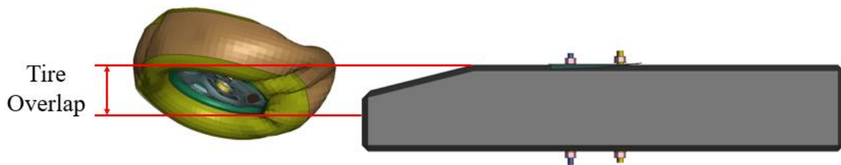
Figure 52. Tire-Buttress Overlap Measurement
