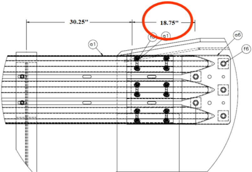
Figure 17. Unsupported Span Length from the As-tested 34-in. Tall AGT
