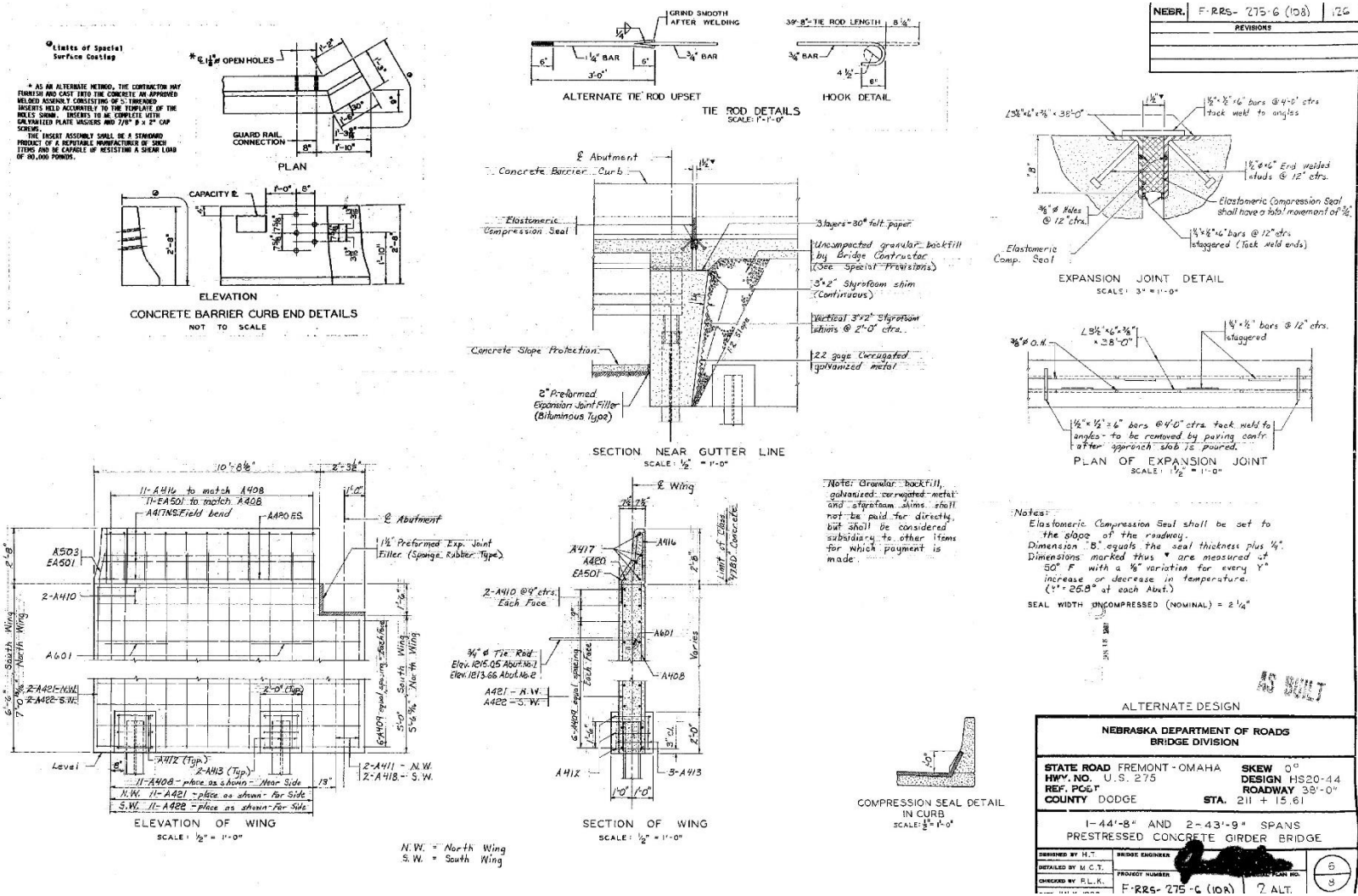
Figure A-9. NDOT Design Details, Buttriss
