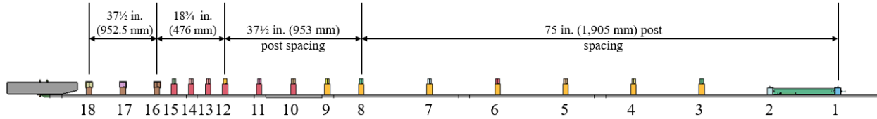
Figure 39. AGT Post Spacing
