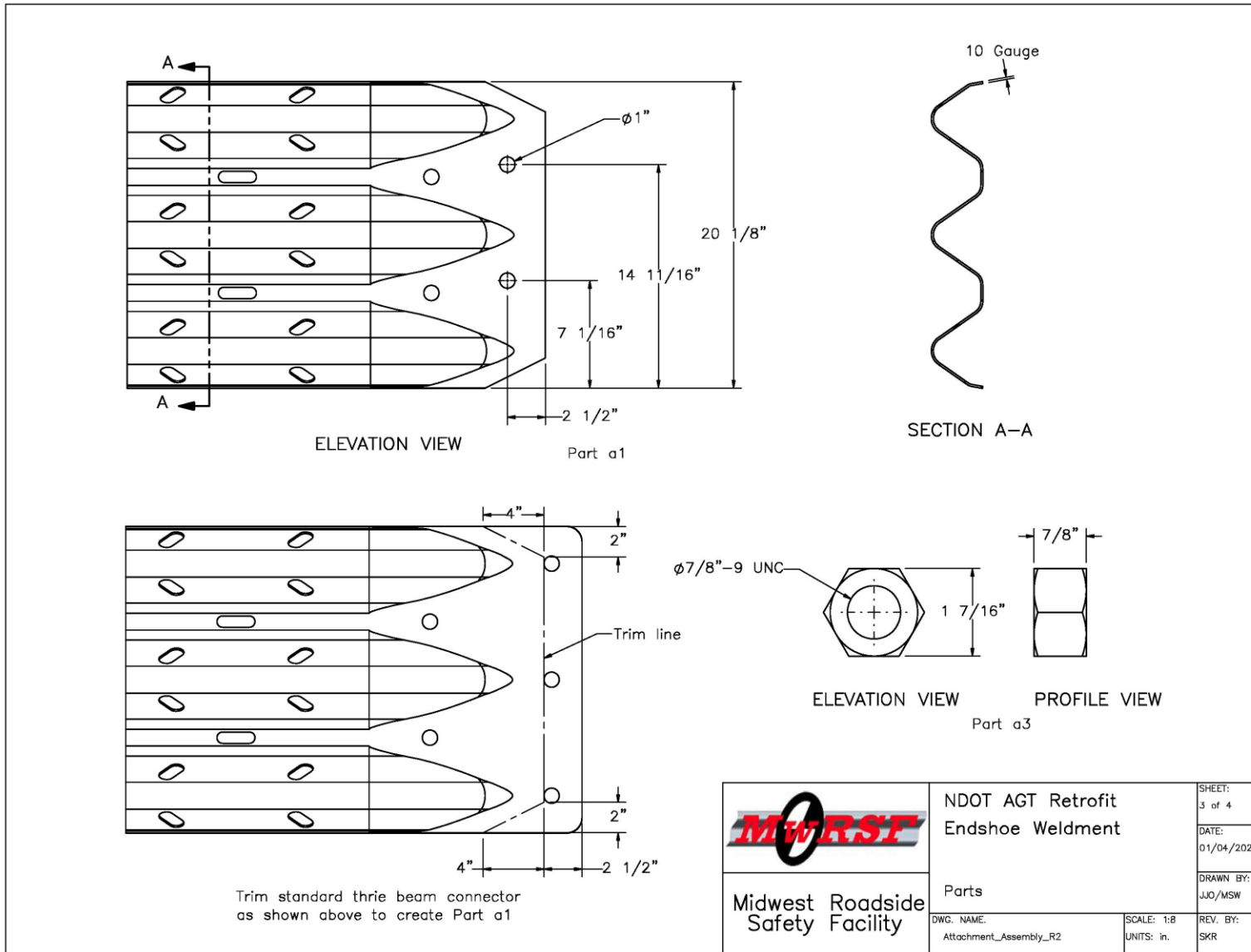
Figure 99. Connector Plate Assembly, Trim Lines for Thrie Beam Terminal Connector
