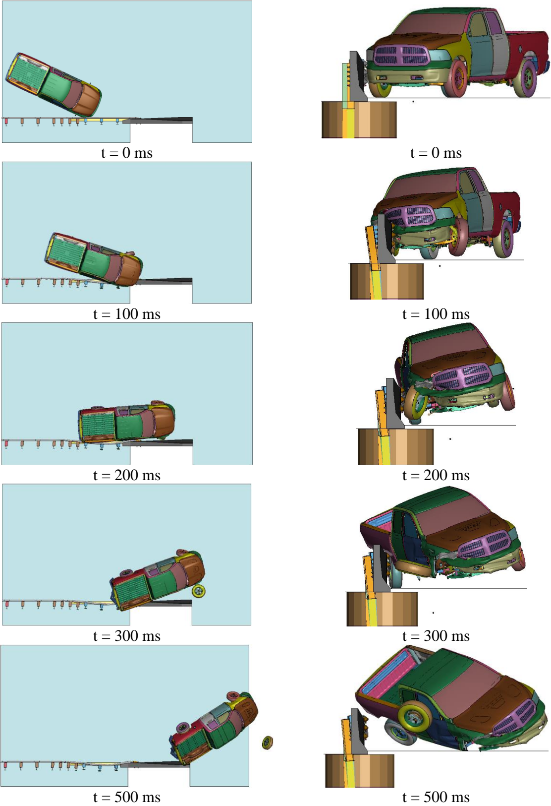
Figure 73. Sequential Images, Simulation No. B8-CP+CB-3N-WD
