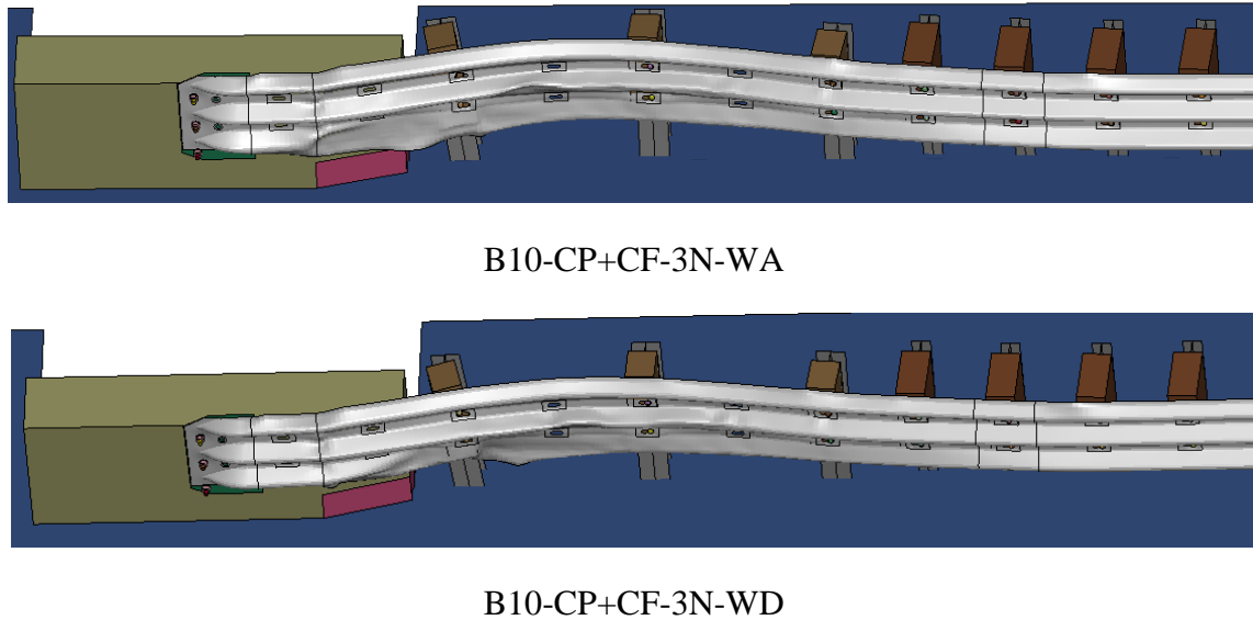
Figure 83. System Damage, Buttress 10
