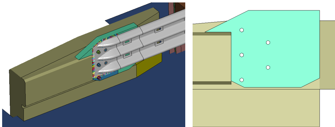
Figure 85. Redesigned Connection Spacer (teal), Buttress 2
