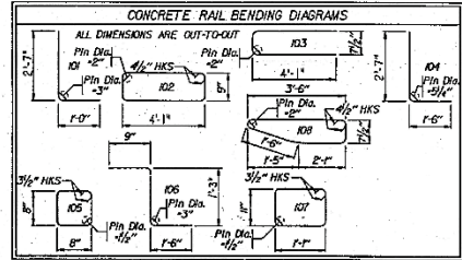
Figure A-3. NDOT Design Details, Buttress 3
