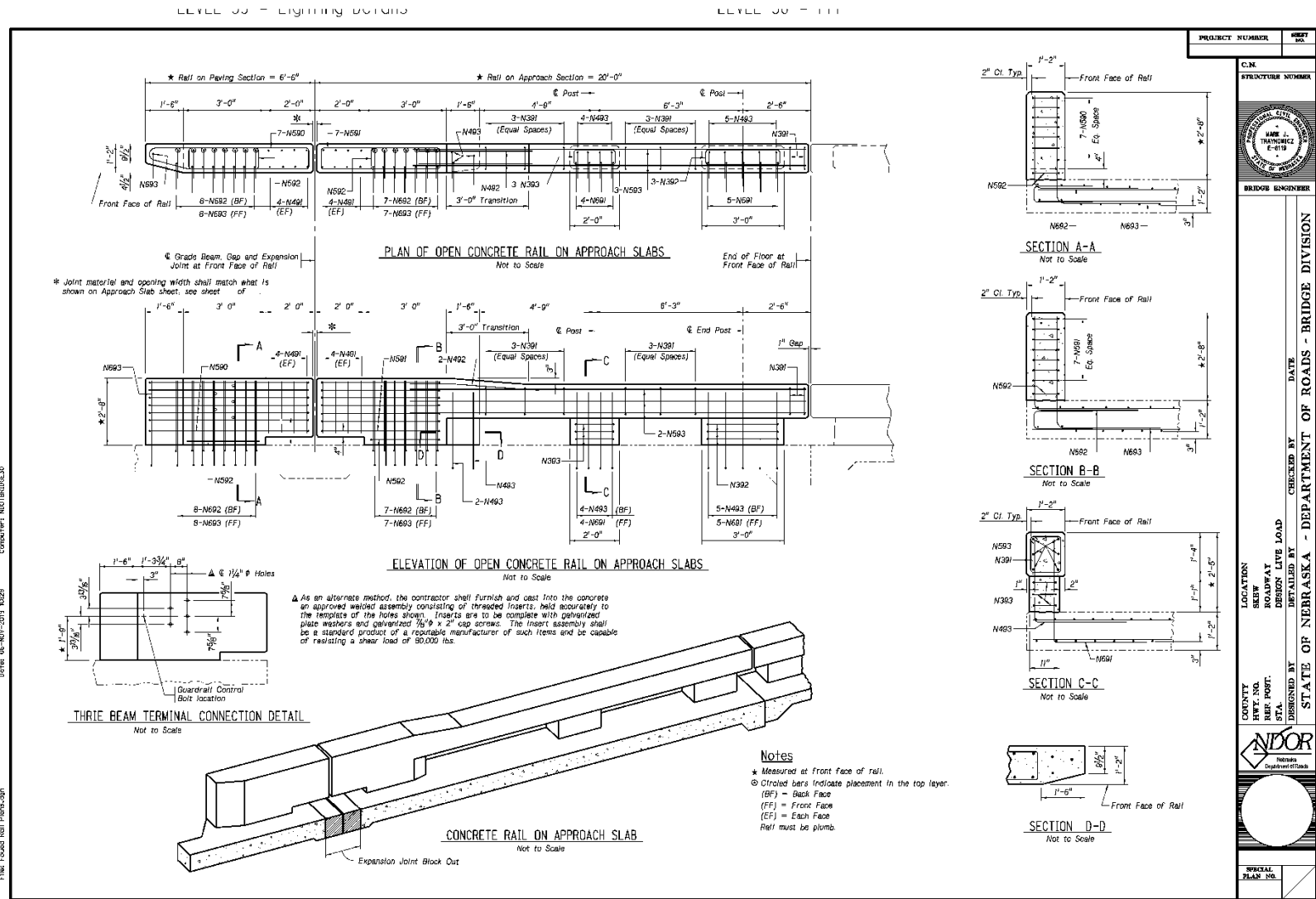
Figure A-5. NDOT Design Details, Buttrass 5
