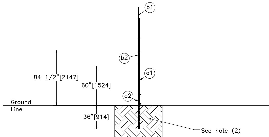
PROFILE VIEW
