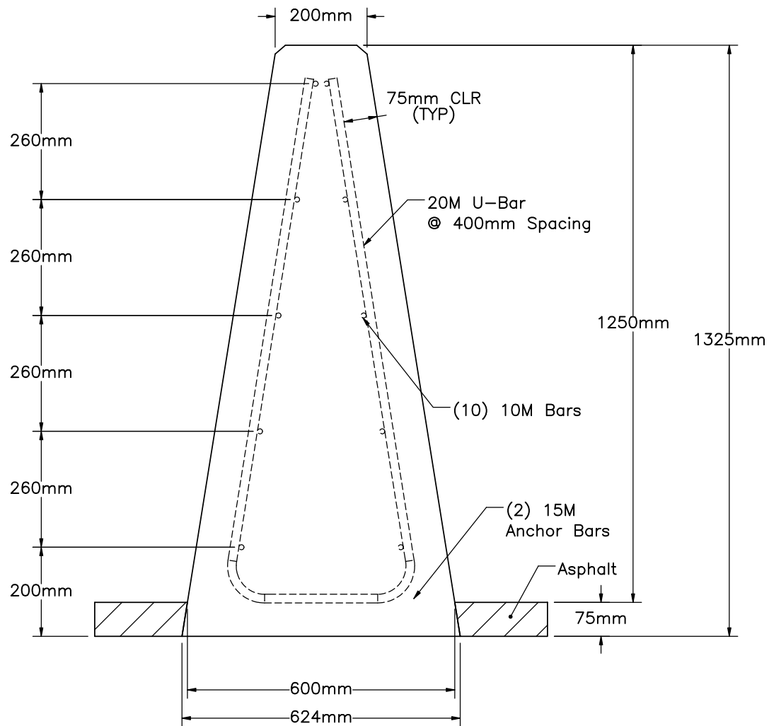
INTERIOR SECTION
