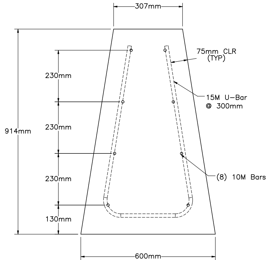
END SECTION
