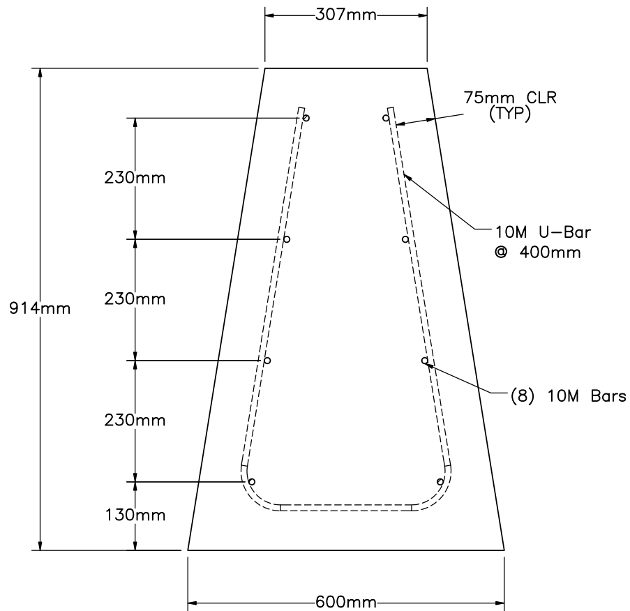
INTERIOR SECTION
