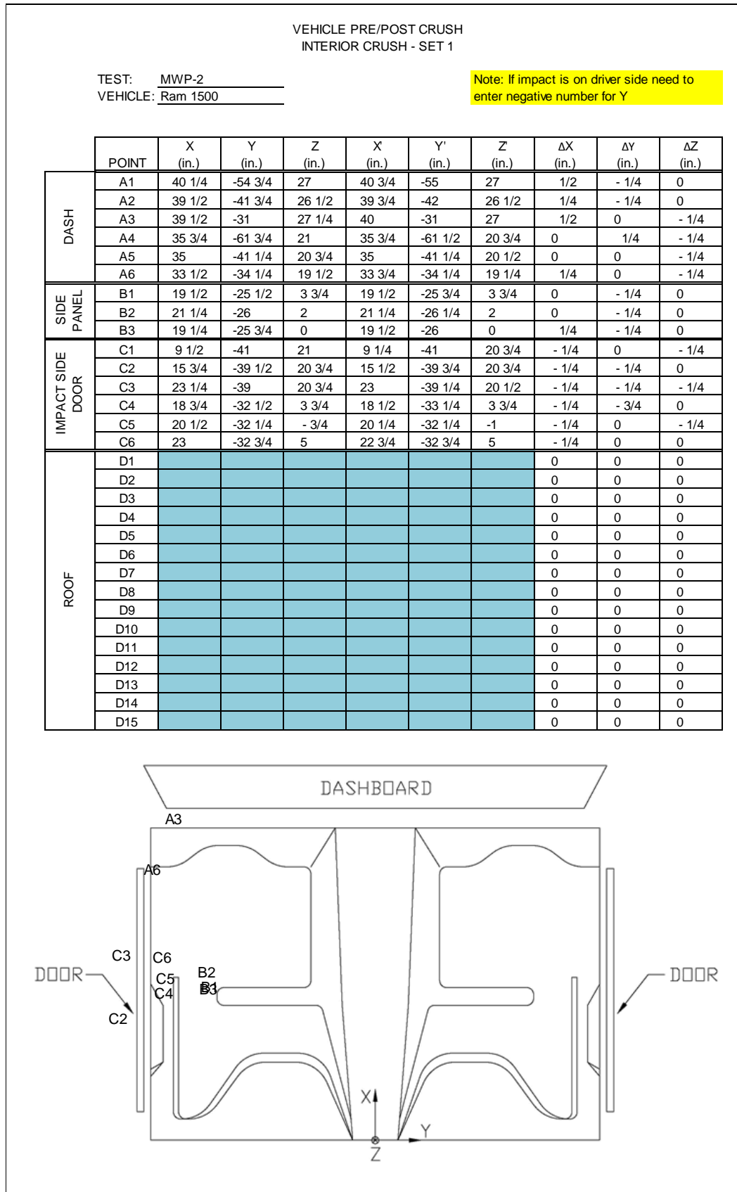
Figure D-9. Occupant Compartment Deformation Data – Set 1, Test No. MWP-2
