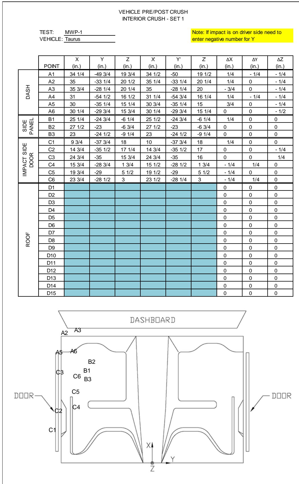
Figure D-3. Occupant Compartment Deformation Data – Set 1, Test No. MWP-1
