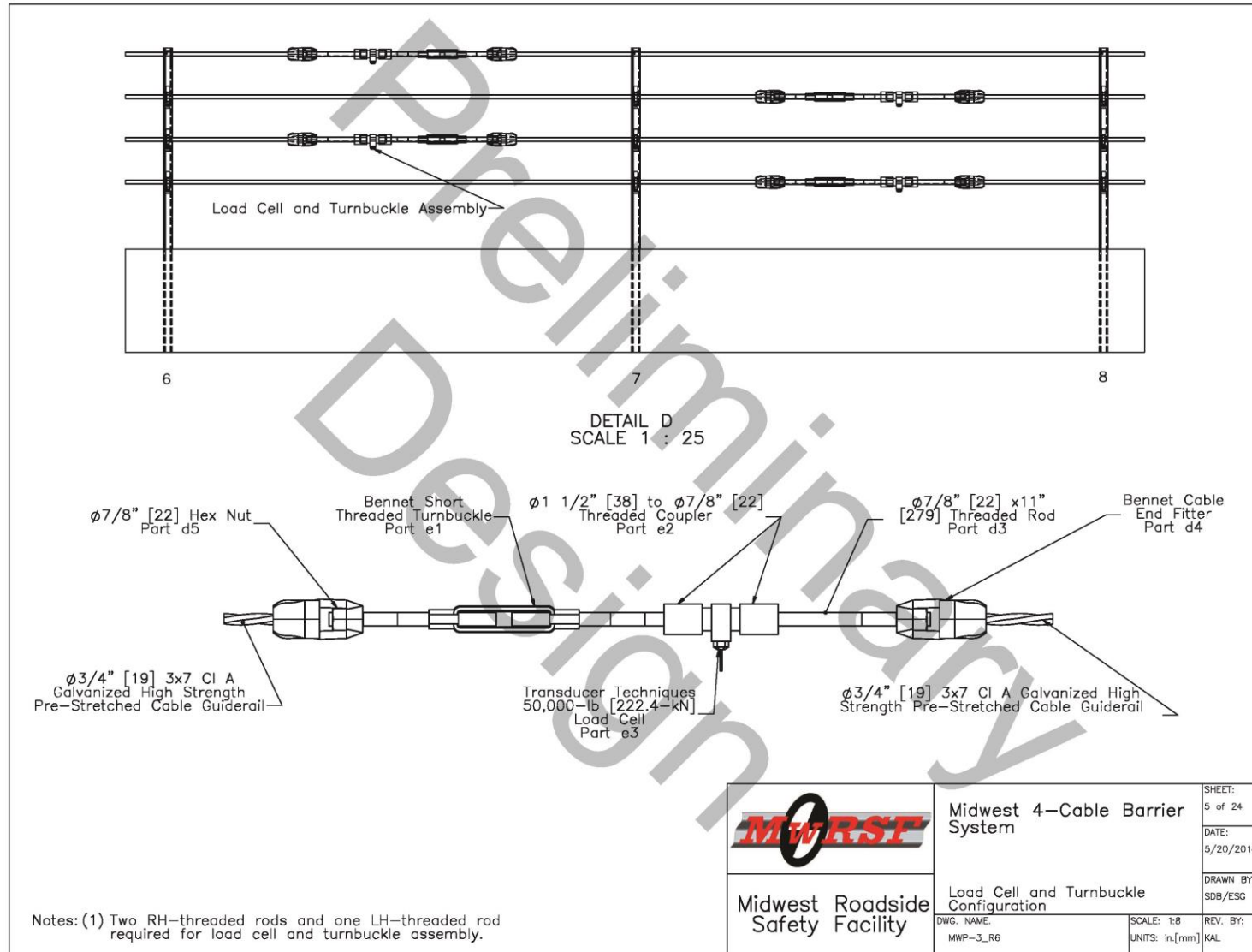
Figure 73. Load Cell and Turnbuckle Configuration, Test No. MWP-3
