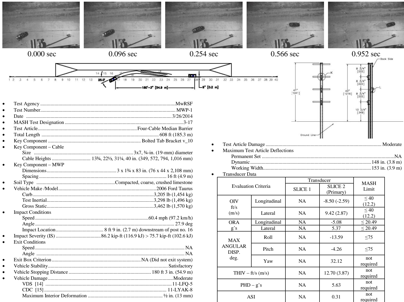
Figure 40. Summary of Test Results and Sequential Photographs, Test No. MWP-1
