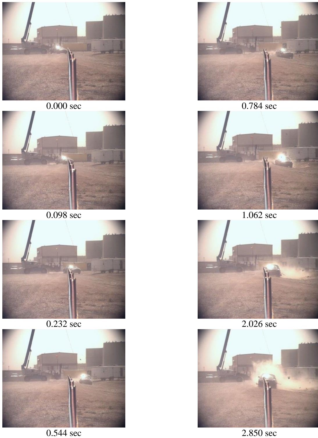
Figure 42. Additional Sequential Photographs, Test No. MWP-1
