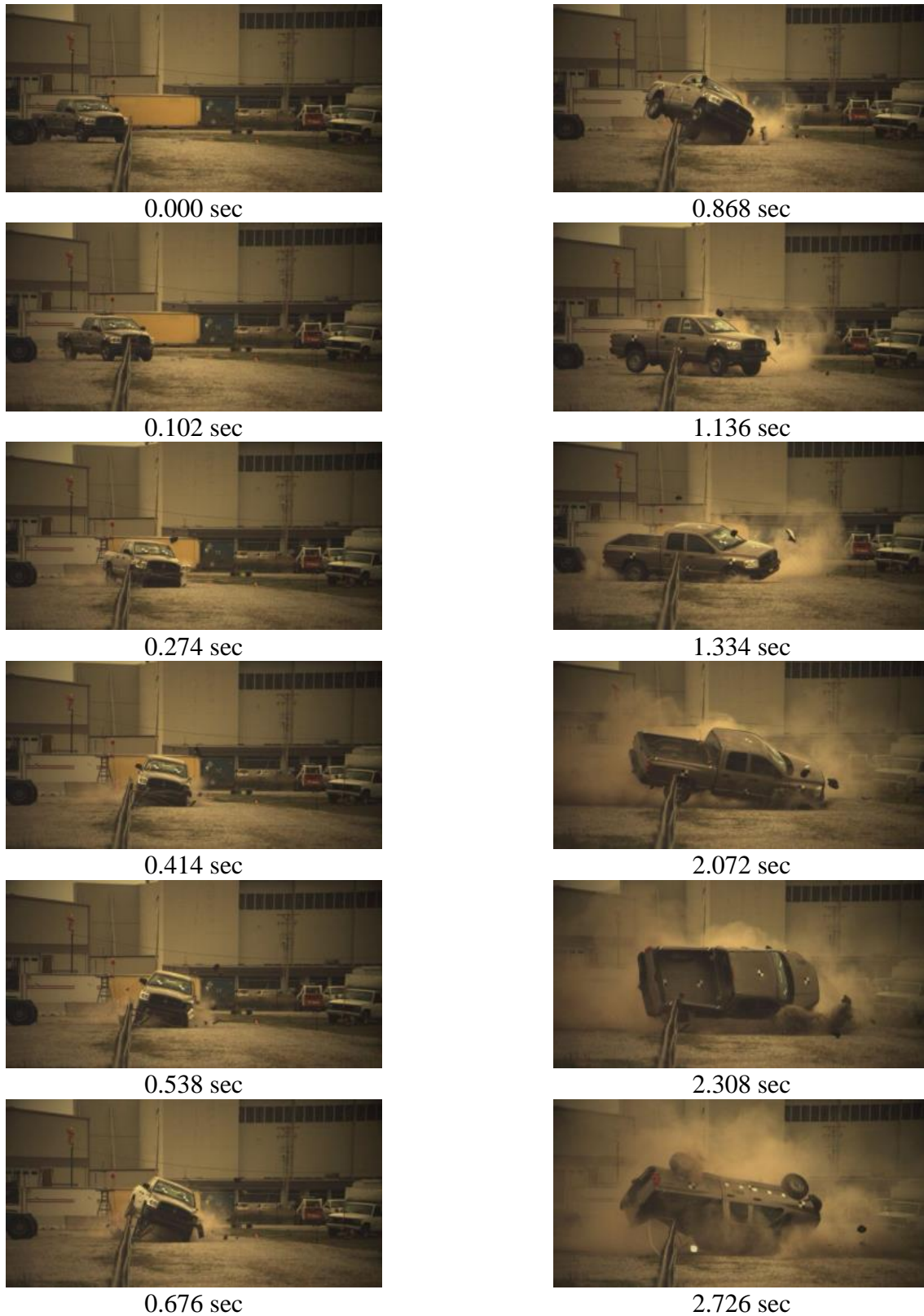
Figure 96. Additional Sequential Photographs, Test No. MWP-3
