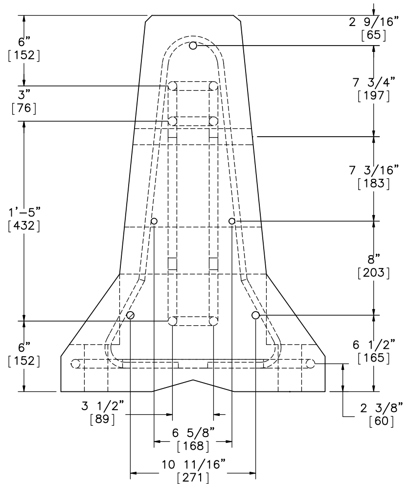
SECTION H-H
