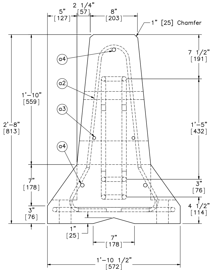
SECTION G-G
