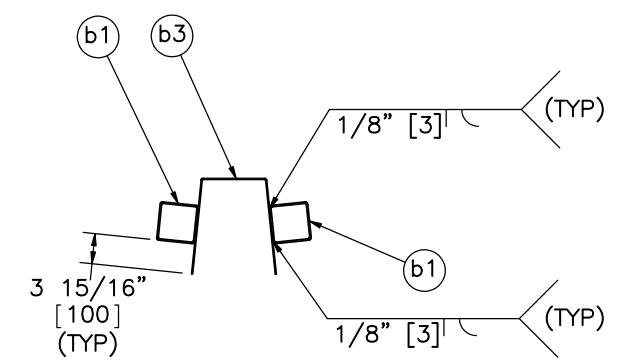
PROFILE VIEW
