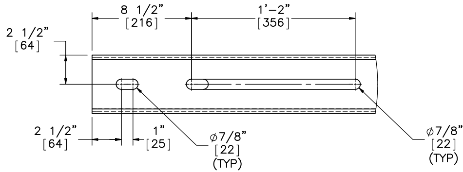
DETAIL I (PLAN VIEW)
