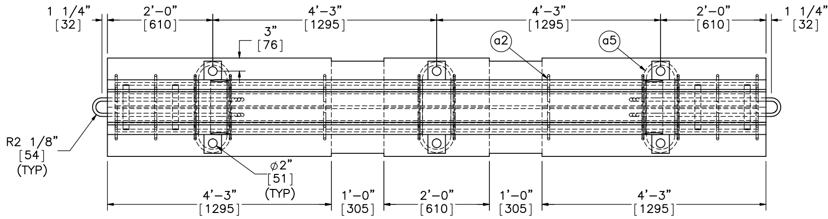
PLAN VIEW
