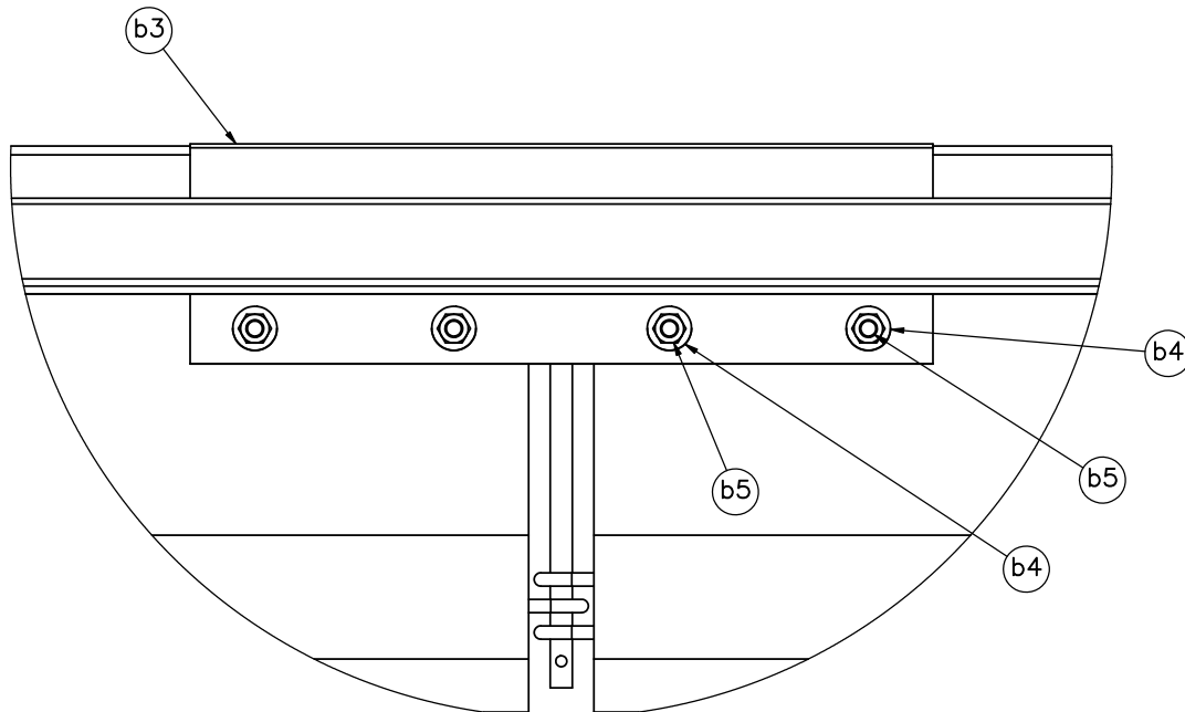
DETAIL D (ELEVATION VIEW)
