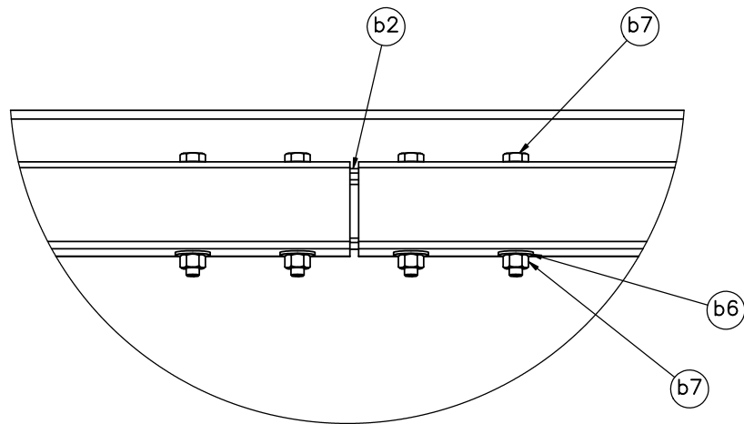
DETAIL F (ELEVATION VIEW)
