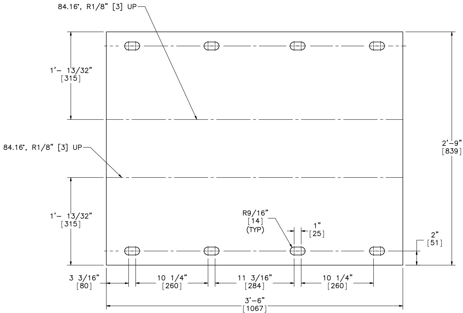
Part b3 (Unbent)
