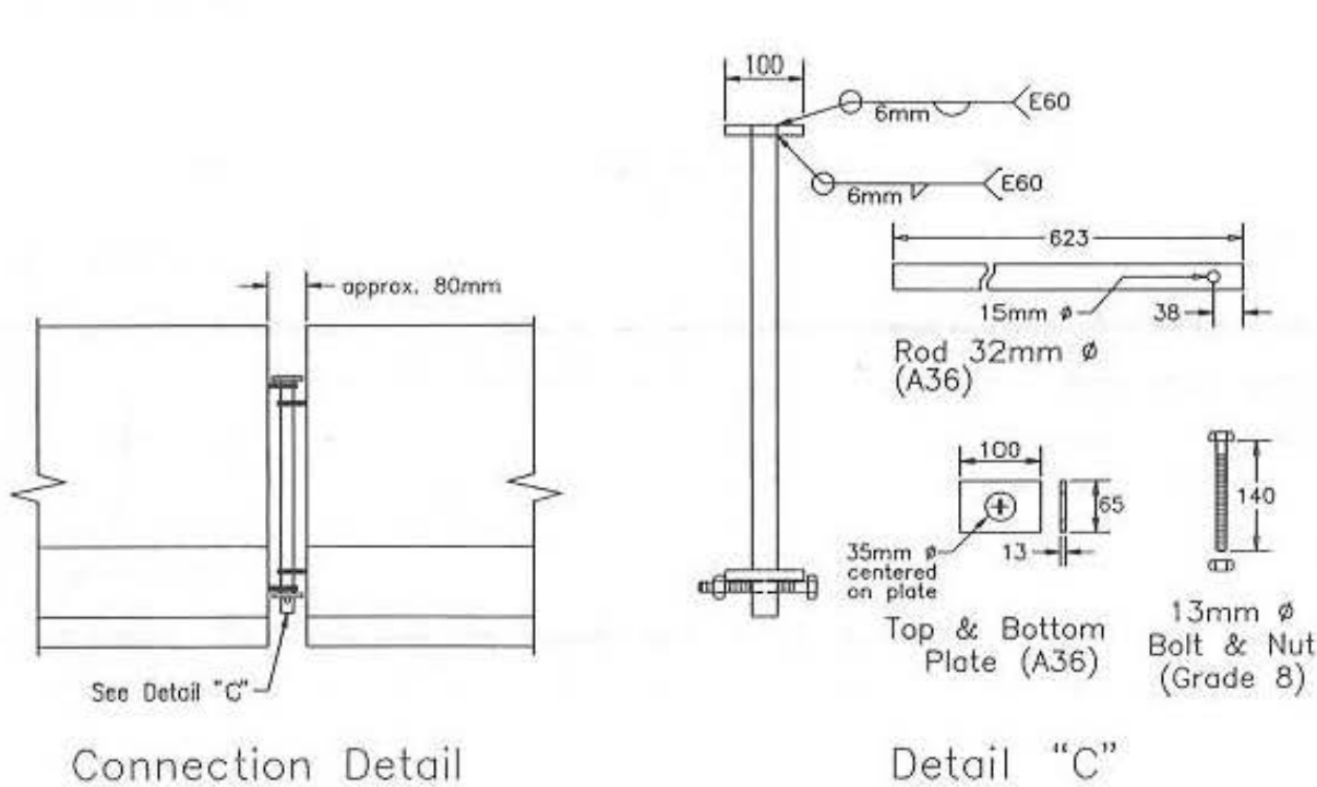
Figure 38. Connection Details, Design No. 3B
