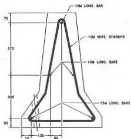
INTERIOR STIRRUP
