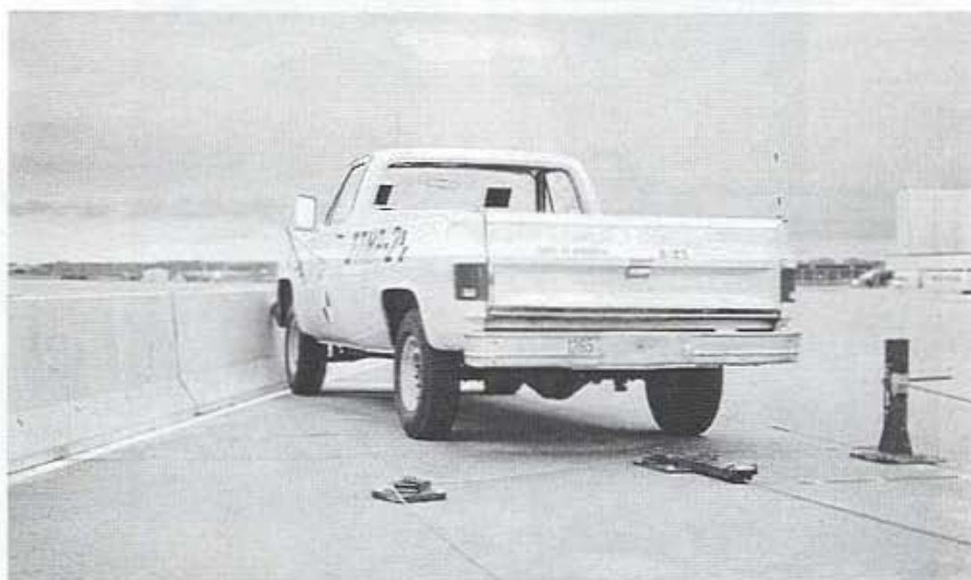
Figure 30. Impact Location, Test ITMP-2
