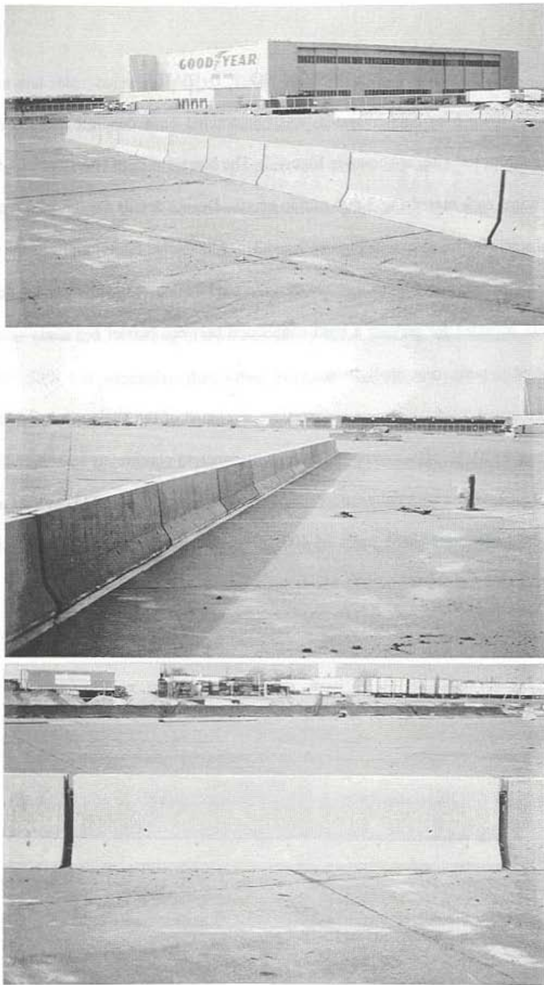
Figure 1. Temporary F-Shape CMB System, Design No. 1
