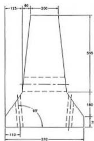
Anchor Hole Placement
