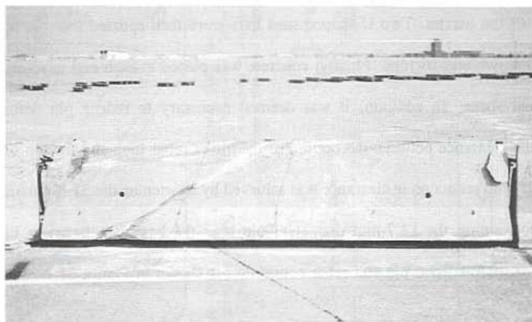
Figure 22. Cracks in Barrier Segment No. 9, Test ITMP-1
