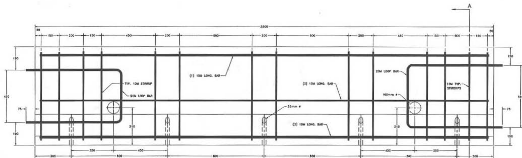
SIDE VIEW
