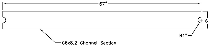
Strut Details
