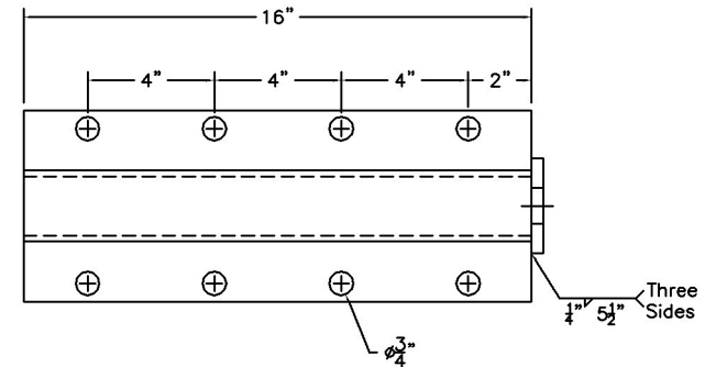
Anchor Bracket (Part c2)
