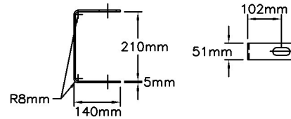
Yoke Details
