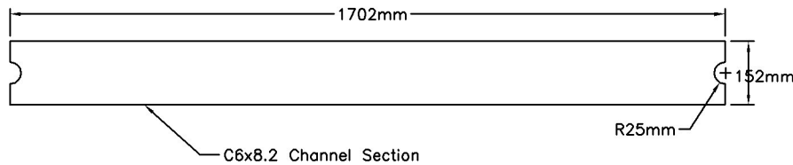
Strut Details
