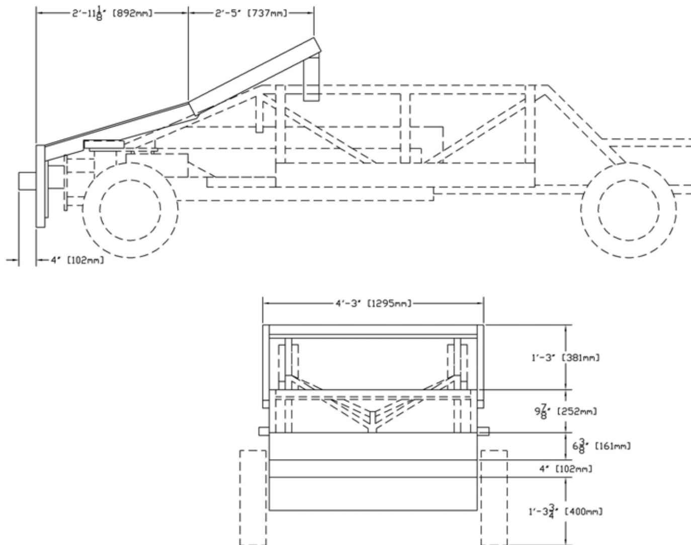
Figure 2. Modified Bogie Vehicle Dimensions
