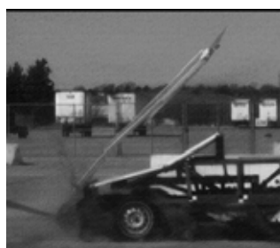
Figure 40. Sequential Photographs – 0 degree orientation, Bogie Test MN6A-0
