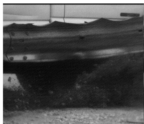
Figure 17. Additional Sequential Photographs, Test 2214MG-1
