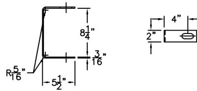
Yoke Details
