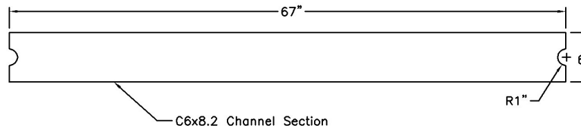
Strut Details
