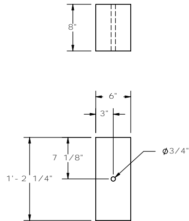
Blockout Part a2
