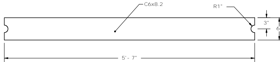
Strut Detail
