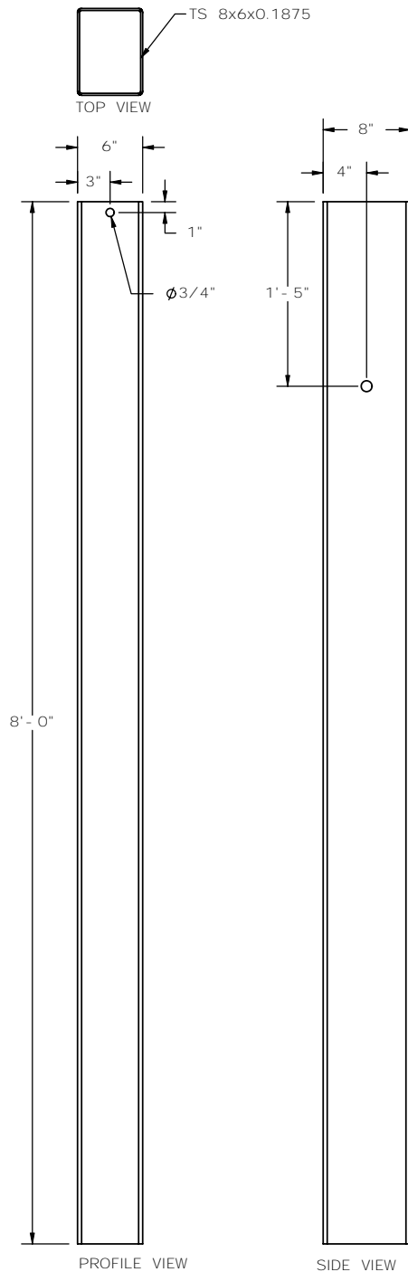
8ft Foundation Tube Part b3
