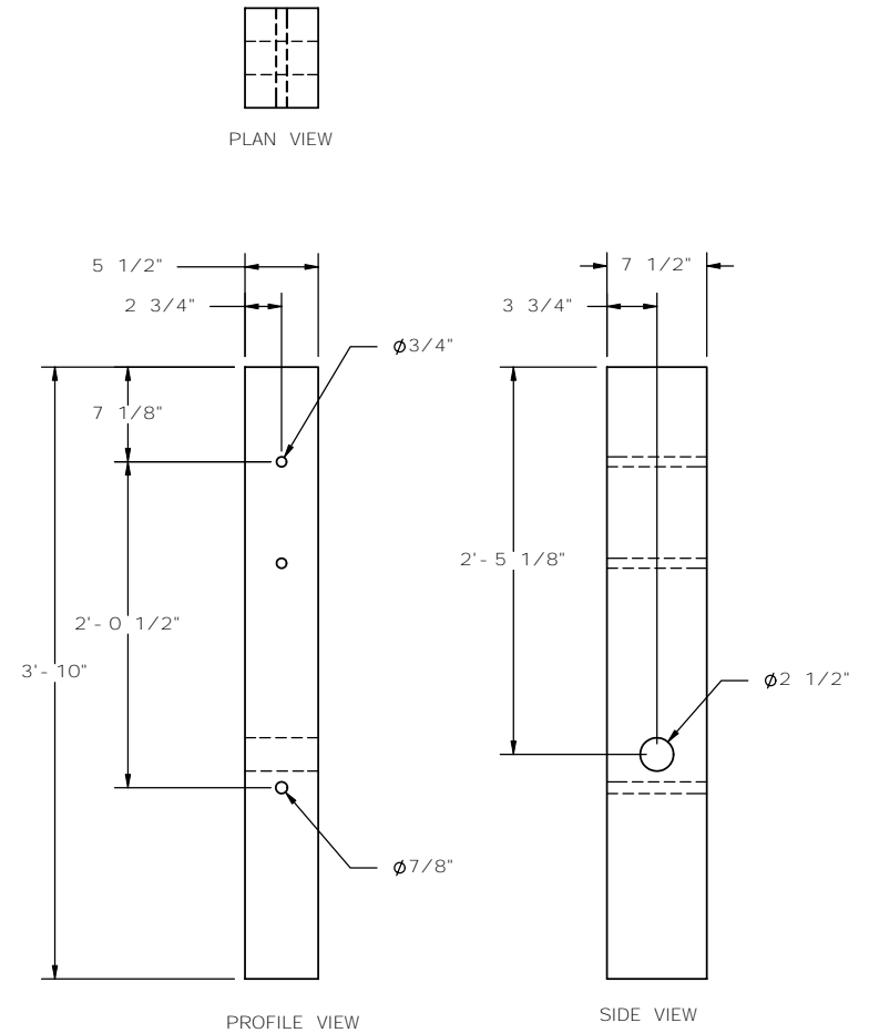
BCT (Thrie) Timber Post Part b2
