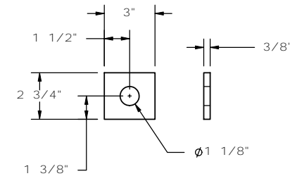
Anchor Bracket Bearing Plate Part c3
