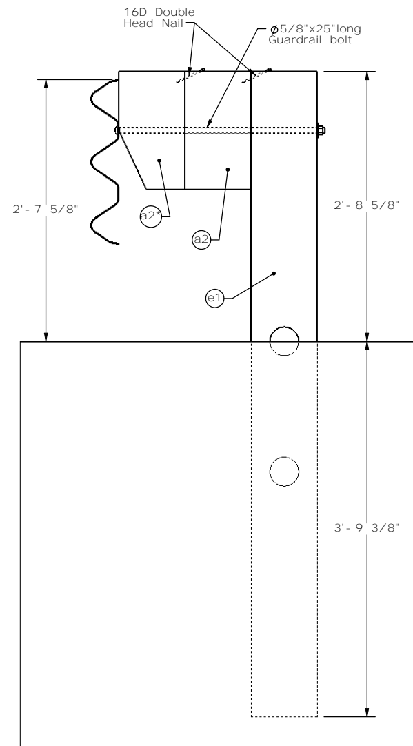
SECTION B-B
