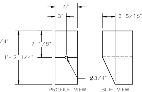
Tapered Blockout Part a2*
