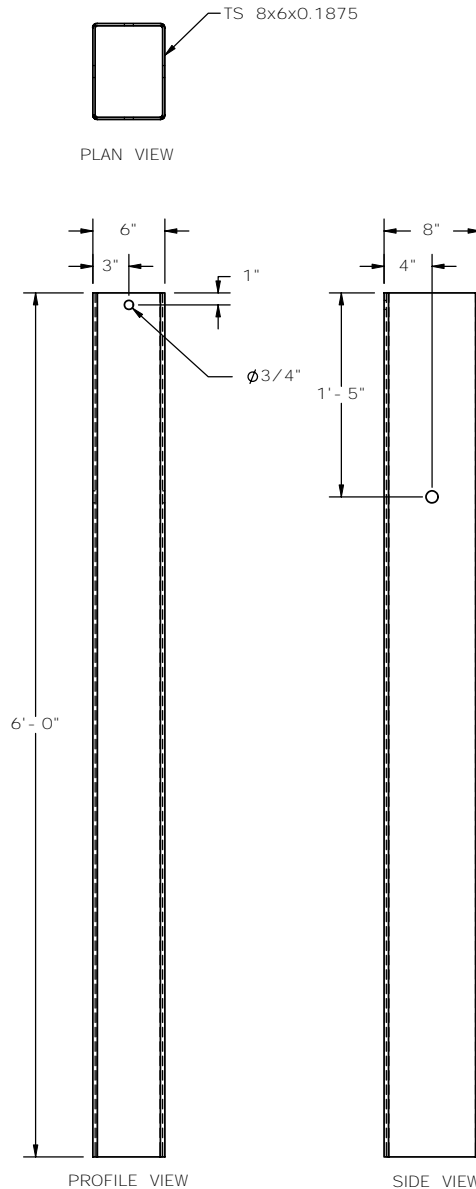
6ft Foundation Tube Part b1
