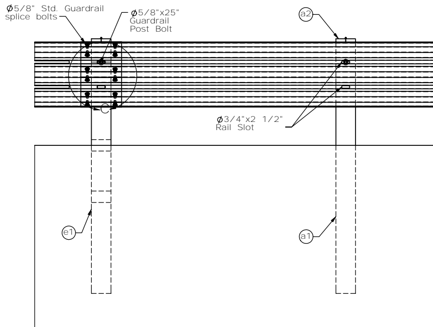
SPLICE DETAIL
