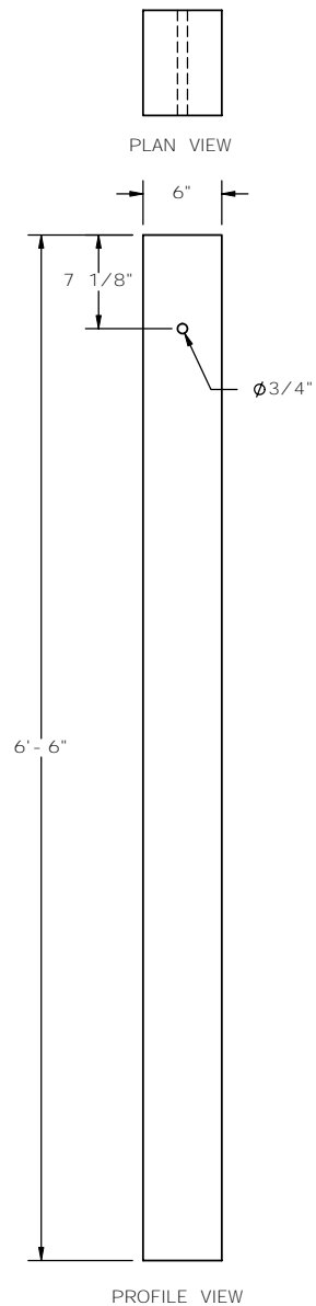
Wood Post Part a1
