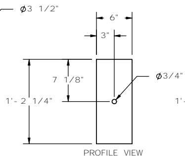
Blockout Part a2
