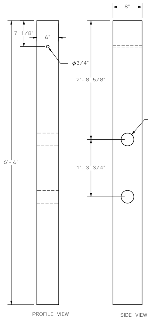
CRT Wood Post Part e1
