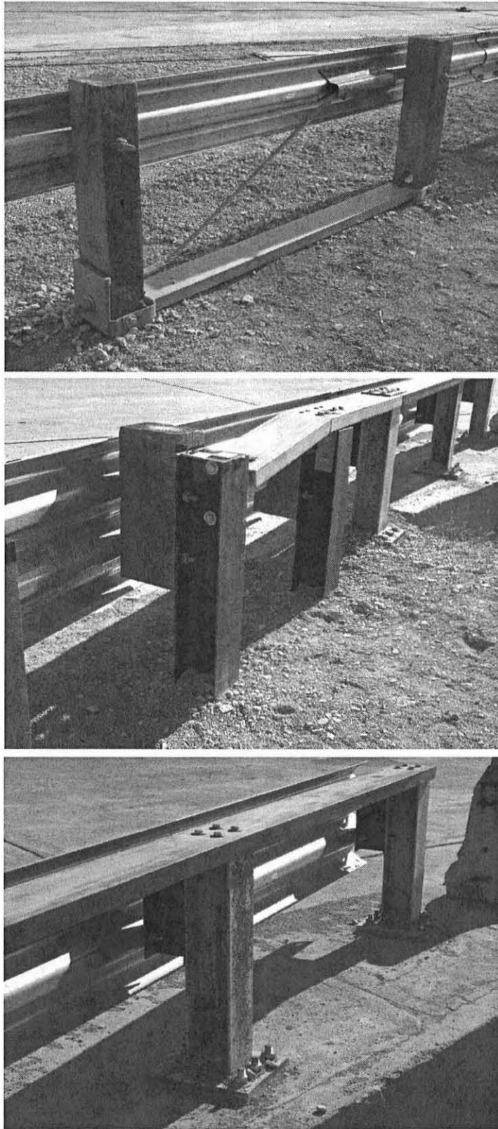
Figure 97. Anchor and Tarmac Connection (Design No. 3)
