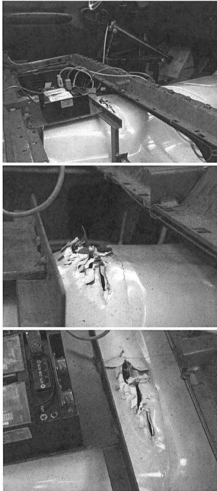
Figure 80. Occupant Compartment Damage, Test MWT-4
