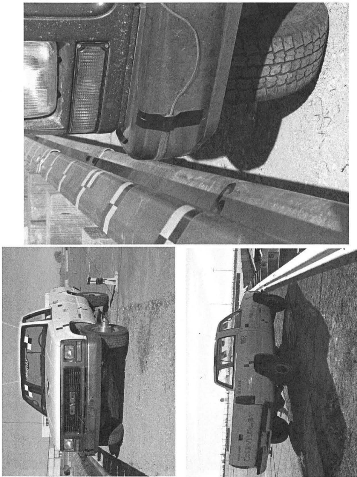
Figure 103. Impact Location, Test MWT-5
