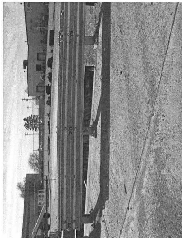
Figure 112. Post Nos. 16 through 21 Damage, Test MWT-5
