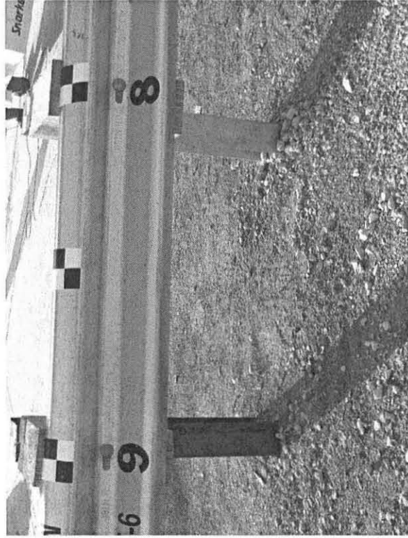
Figure 125. Post Nos. 6 through 9 Damage, Test MWT-6
