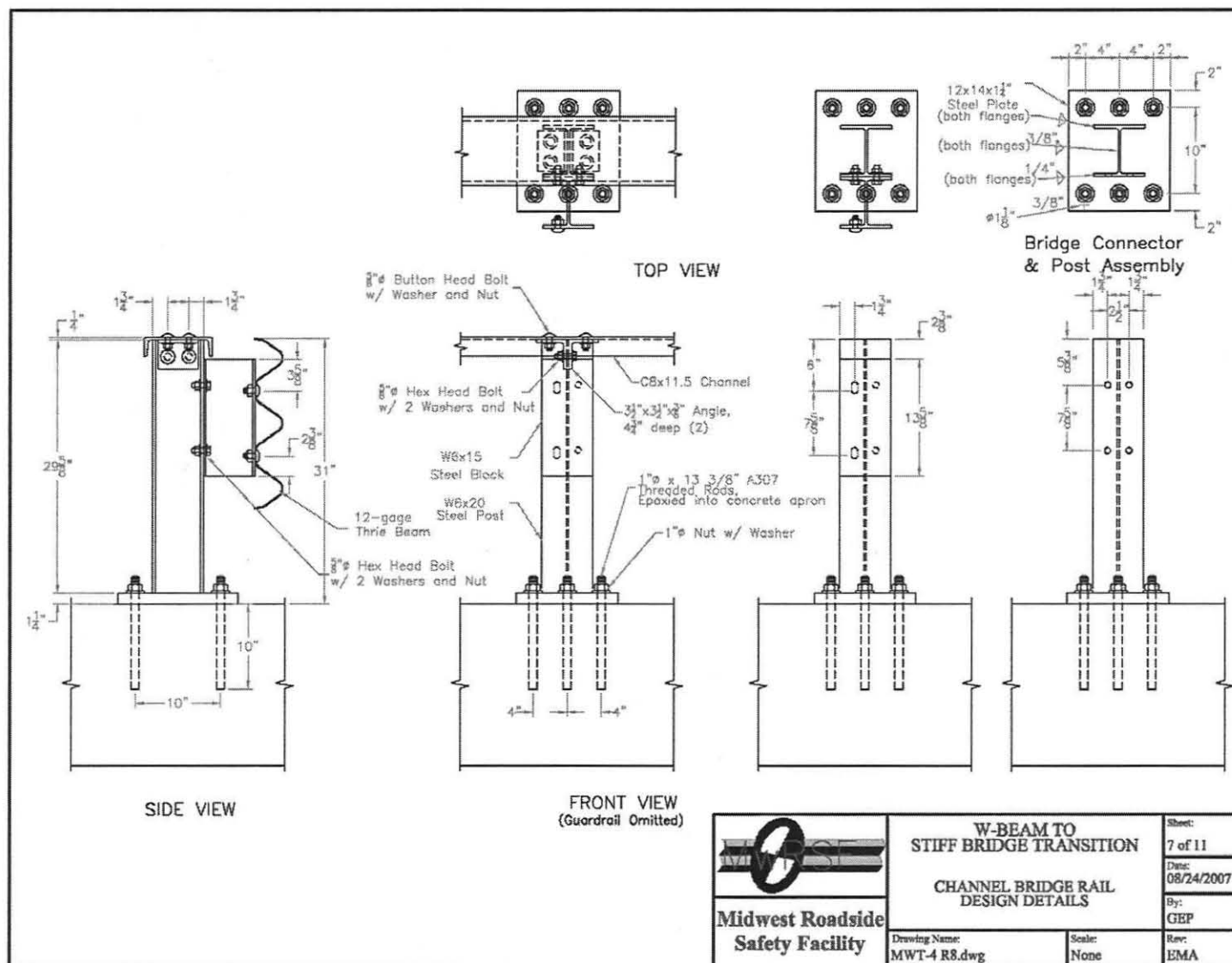
Figure E-7. Channel Bridge Rail Design Details, Design No. 2 (English)
