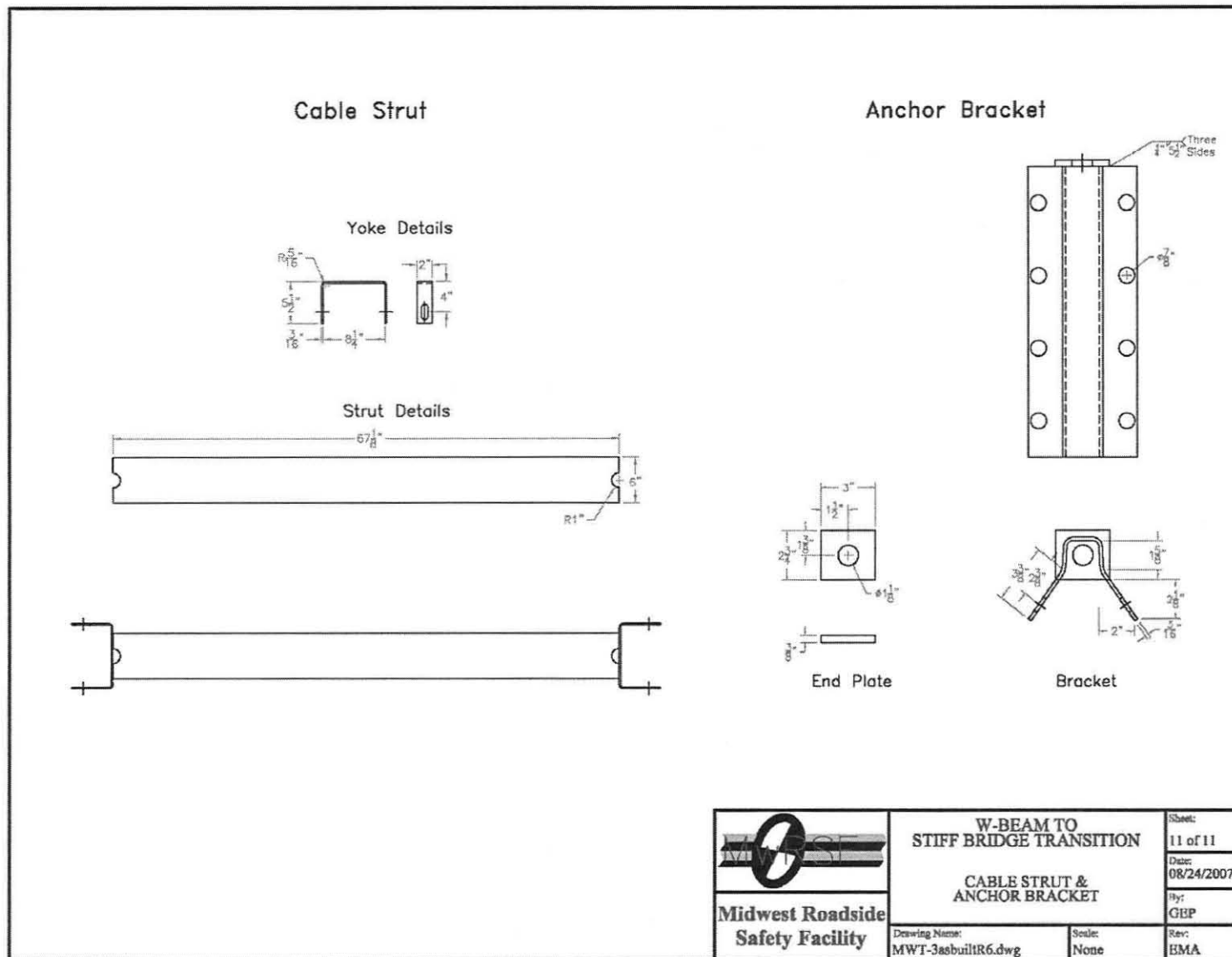
Figure A-11. Cable Strut and Anchor Bracket Details, Design No. 1 (English)
