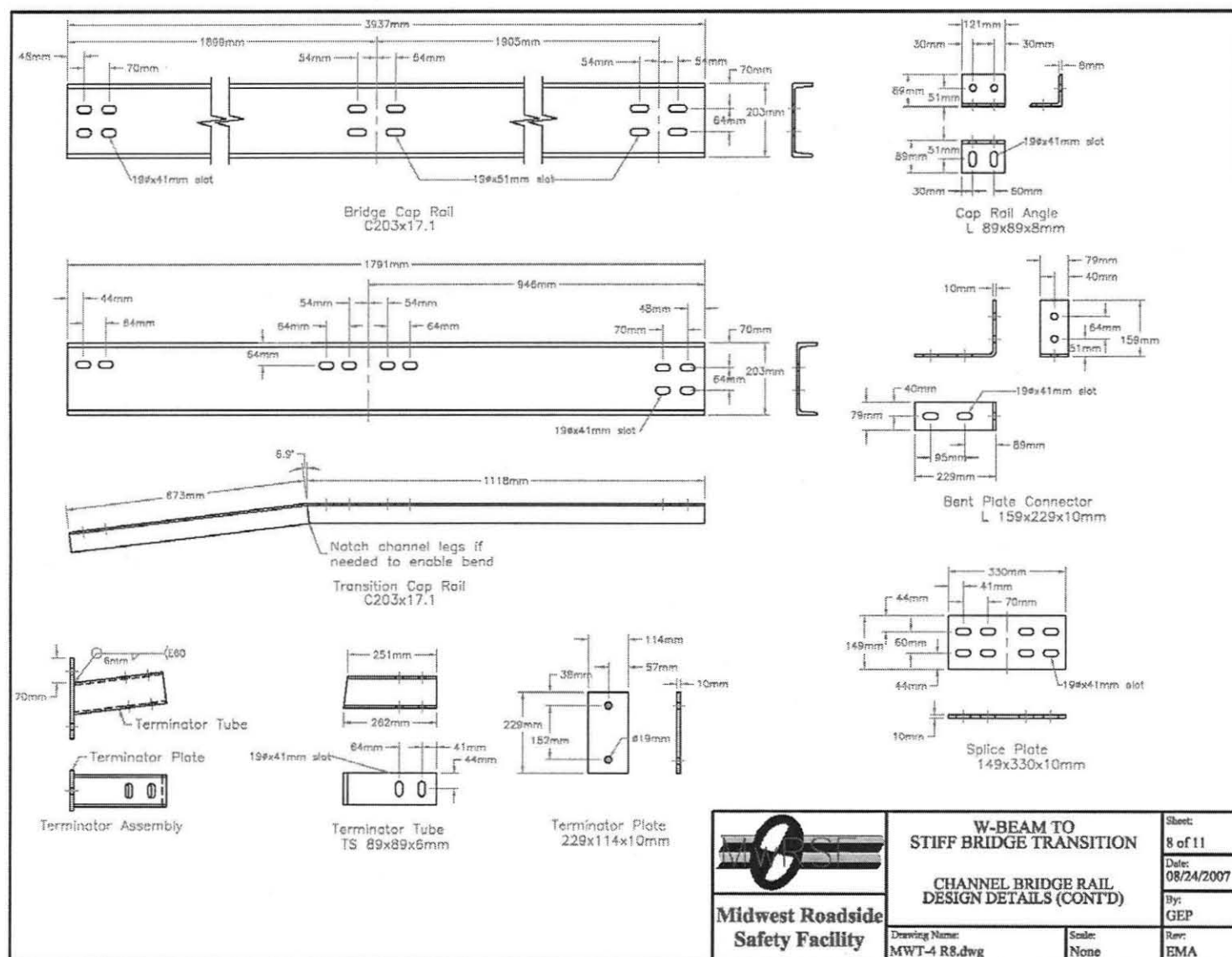
Figure 57. Channel Bridge Rail Design Details (Design No. 2)
