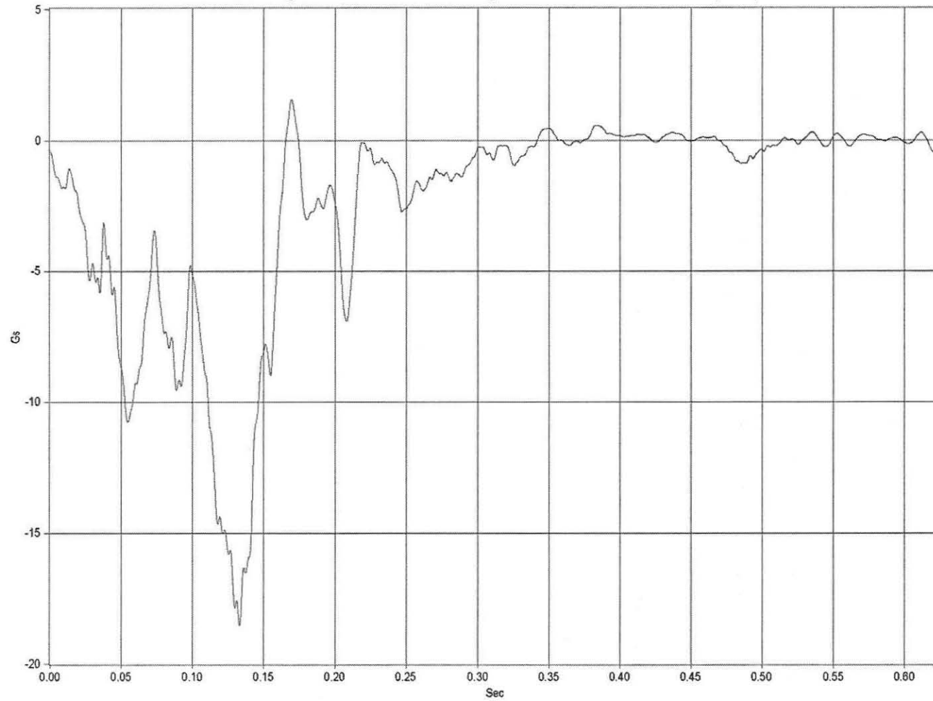
W17: Longitudinal Deceleration - 10-Msec Avg. - CFC 180 Filtered Data - Test MWT-6 (EDR-3)
