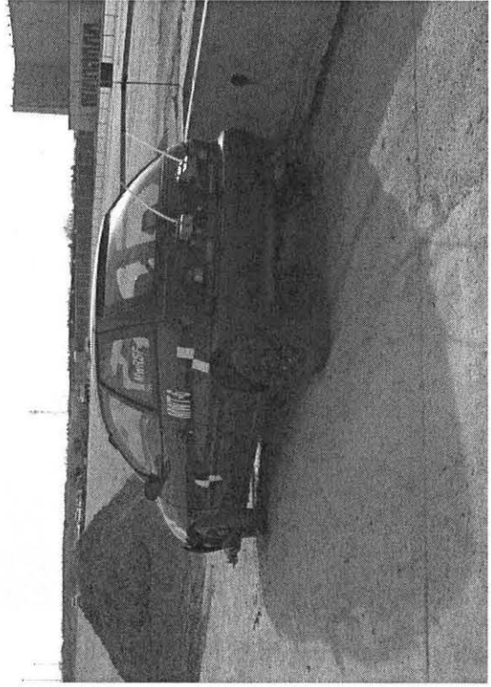
Figure 122. Final Location and Trajectory Marks, Test MWT-6
