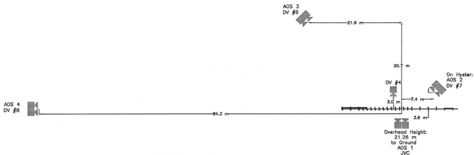
MWT-5 Camera Summary
