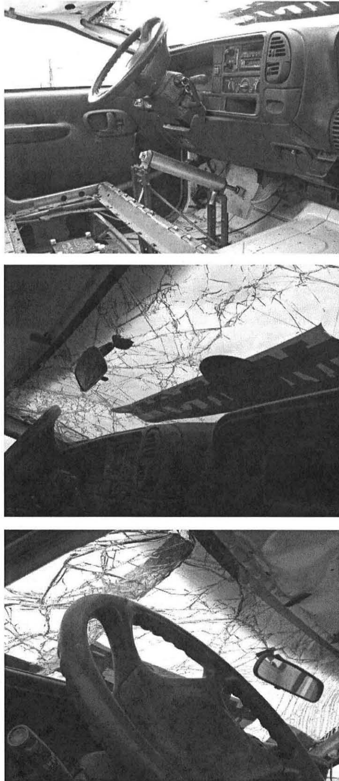
Figure 49. Occupant Compartment and Windshield Damage, Test MWT-3
