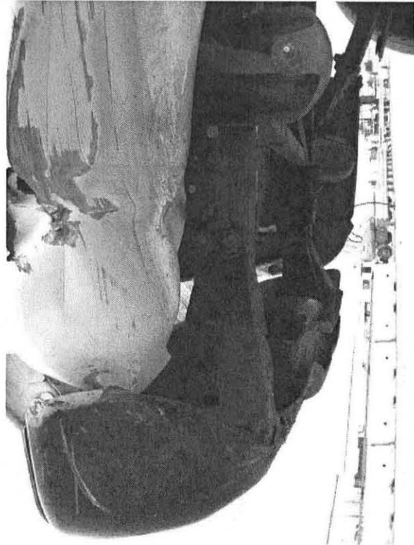
Figure 48. Vehicle Damage, Test MWT-3
