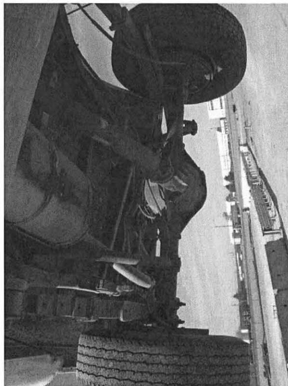
Figure 114. Vehicle Damage, Test MWT-5
