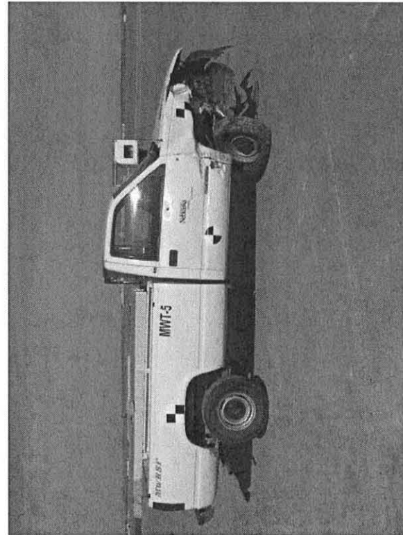
Figure 113. Vehicle Damage, Test MWT-5
