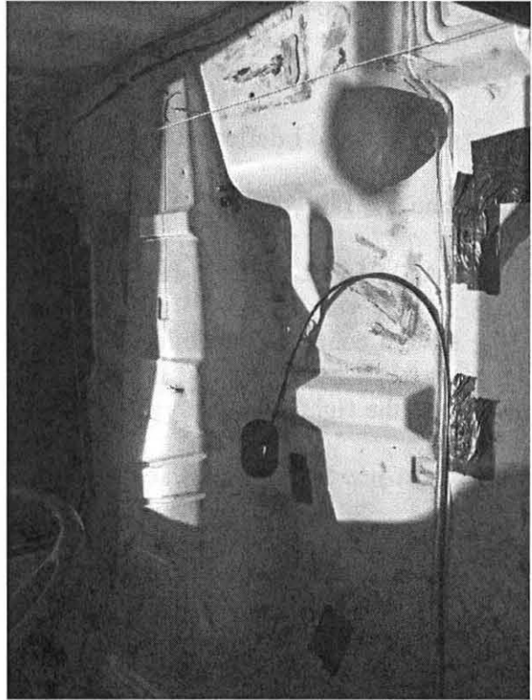
Figure 115. Occupant Compartment Damage, Test MWT-5
