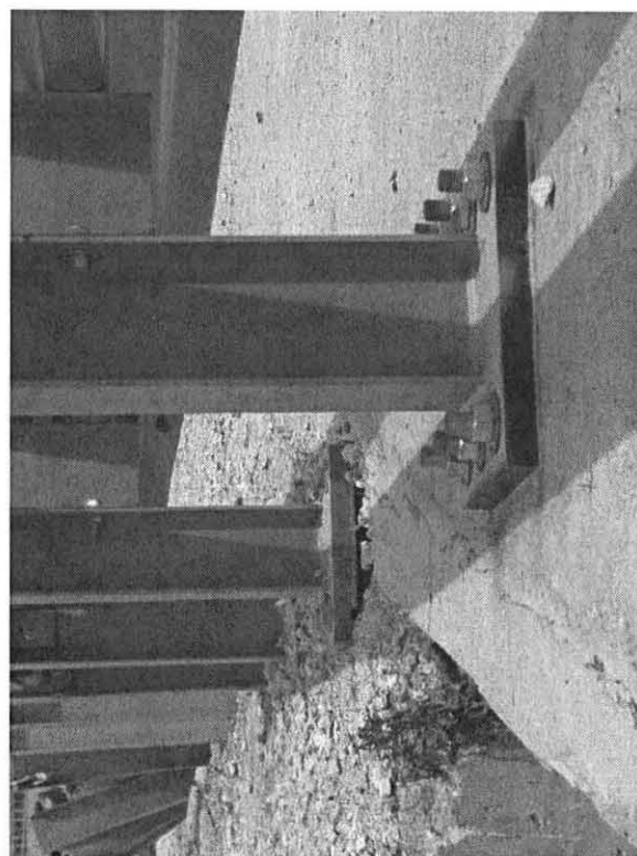
Figure 45. Bridge Posts and Post No. 15 Damage, Test MWT-3
