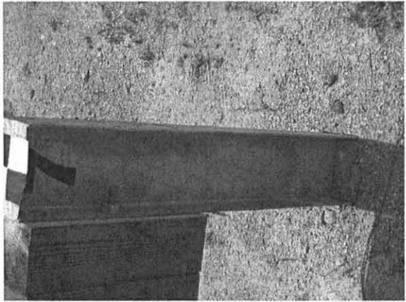
Figure 74. Post Nos. 7 through 9 Damage, Test MWT-4
