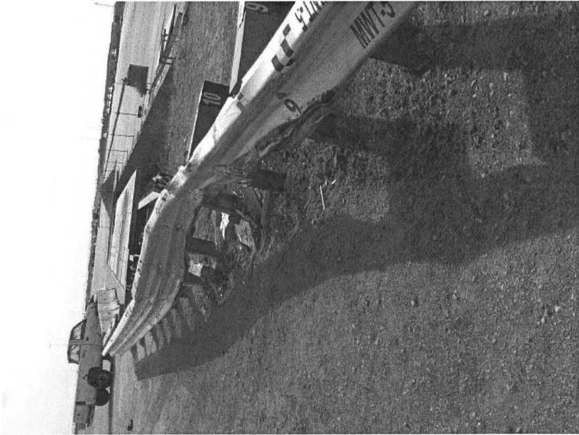
Figure 106. System Damage, Test MWT-5
