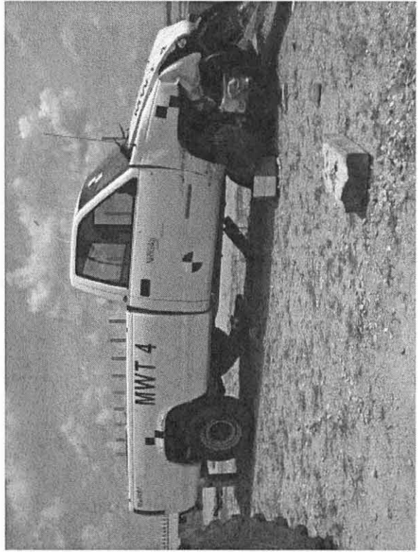
Figure 77. Vehicle Damage, Test MWT-4
