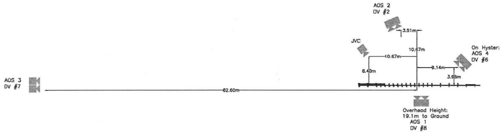
MWT-6 Camera Summary
