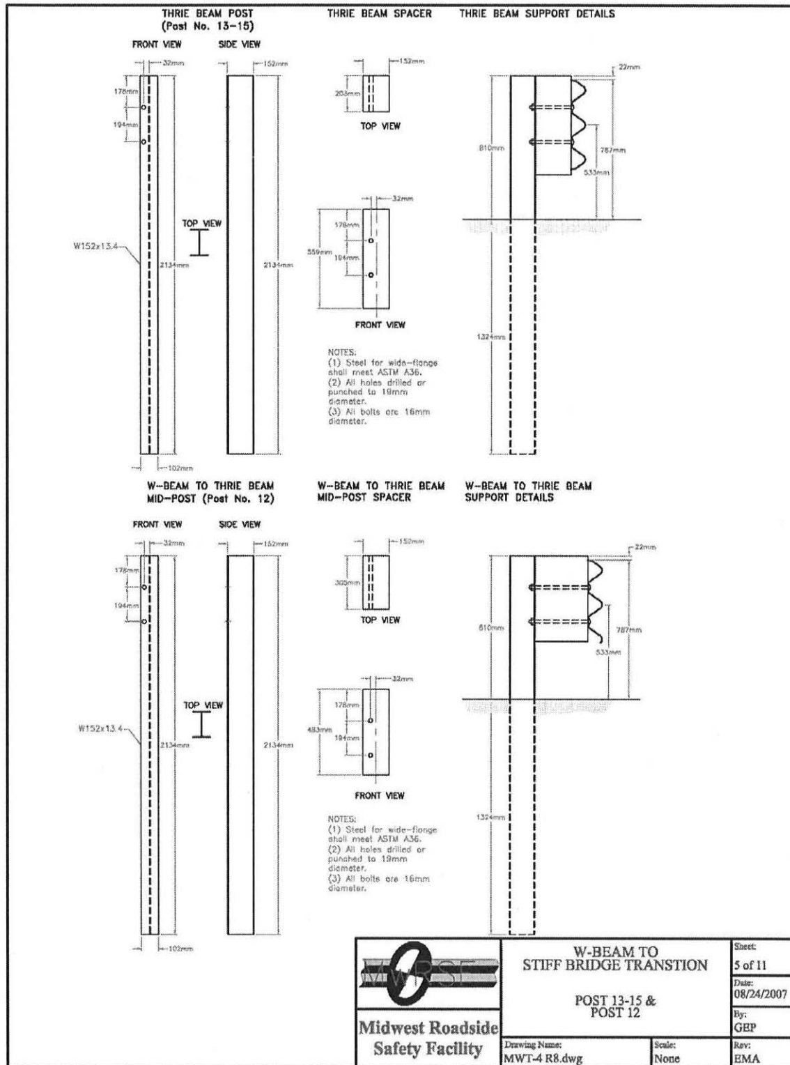
Figure 54. Post Nos. 12 through 15 Details (Design No. 2)
