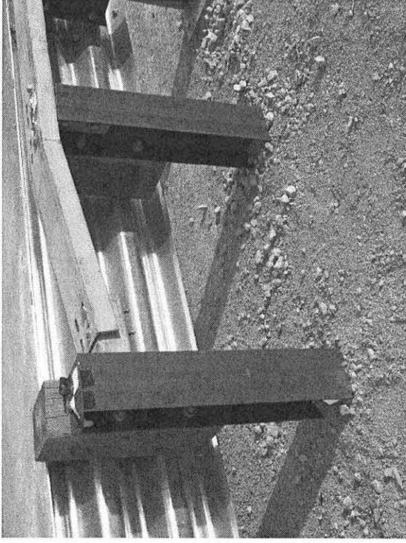
Figure 128. Post Nos. 14 through 19 Damage, Test MWT-6
