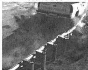
Figure 100. Additional Sequential Photographs, Test MWT-5
