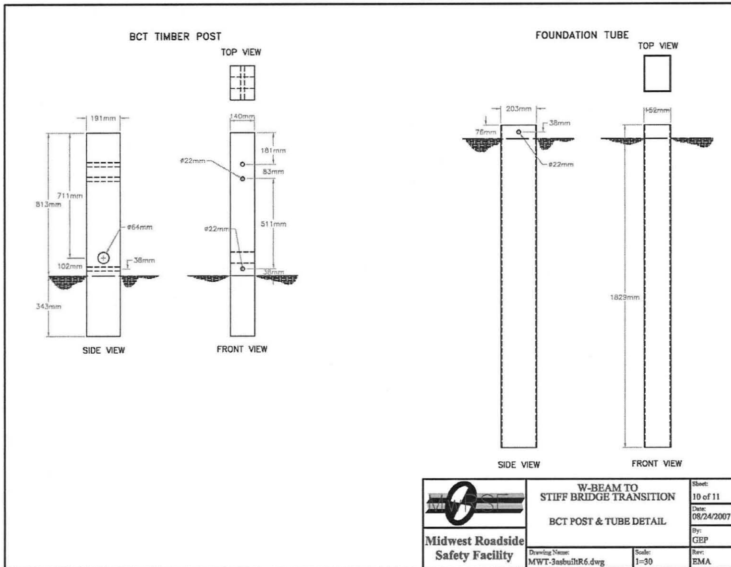
Figure 11. BCT Post and Tube Details (Design No. 1)
