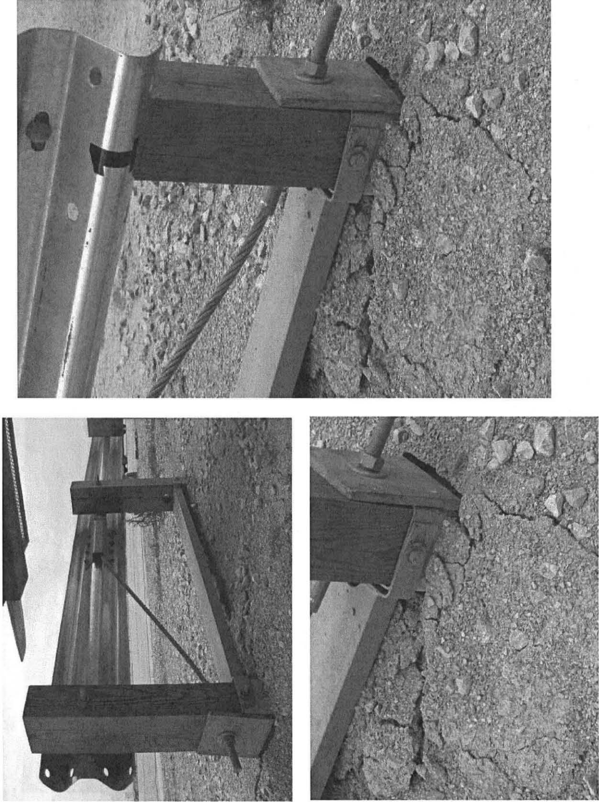
Figure 41. Anchorage Damage, Test MWT-3
