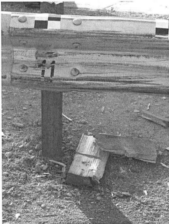
Figure 126. Post Nos. 10 and 11 Damage, Test MWT-6
