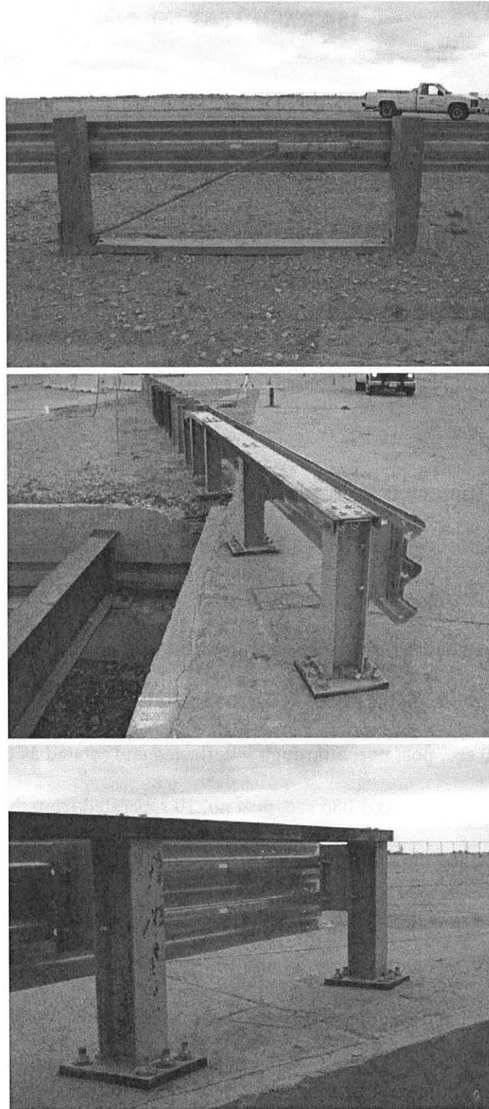
Figure 62. Anchor and Tarmac Connection (Design No. 2)
