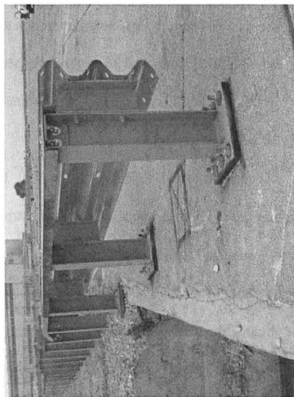
Figure 14. Anchor and Tarmac Connection Details (Design No. 1)
