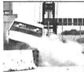
Figure 64. Additional Sequential Photographs, Test MWT-4
