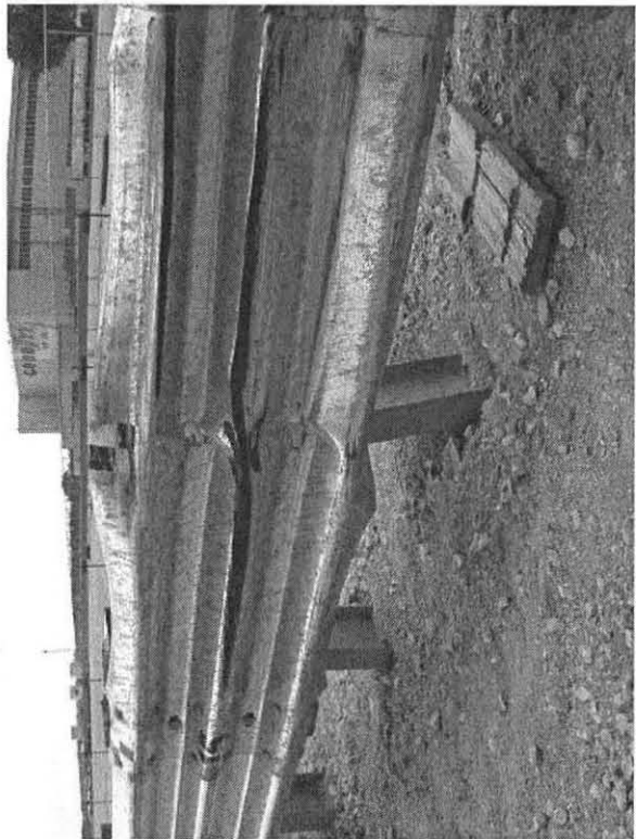
Figure 44. Post Nos. 13 and 14 Damage, Test MWT-3
