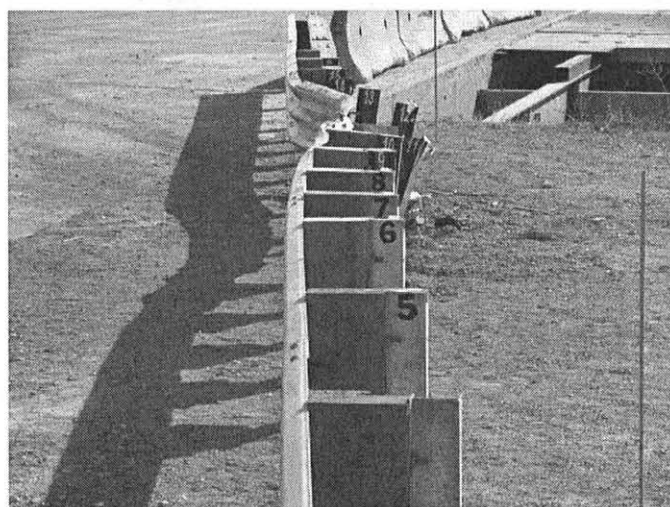
Figure 105. System Damage, Test MWT-5
