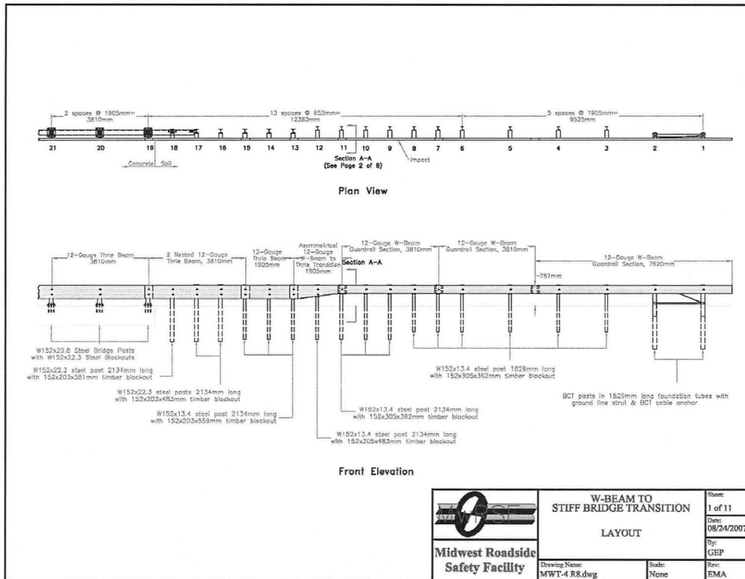
Figure 50. Layout (Design No. 2)
