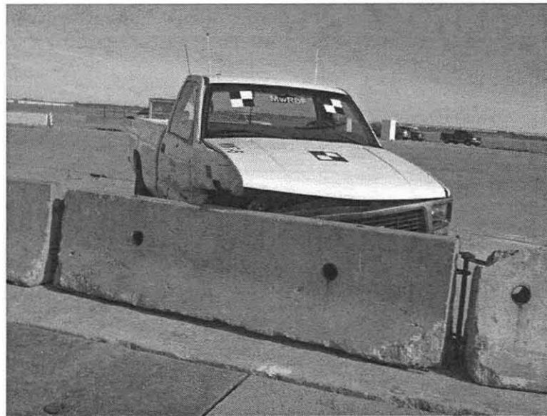
Figure 104. Vehicle Final Position and Trajectory Marks, Test MWT-5
