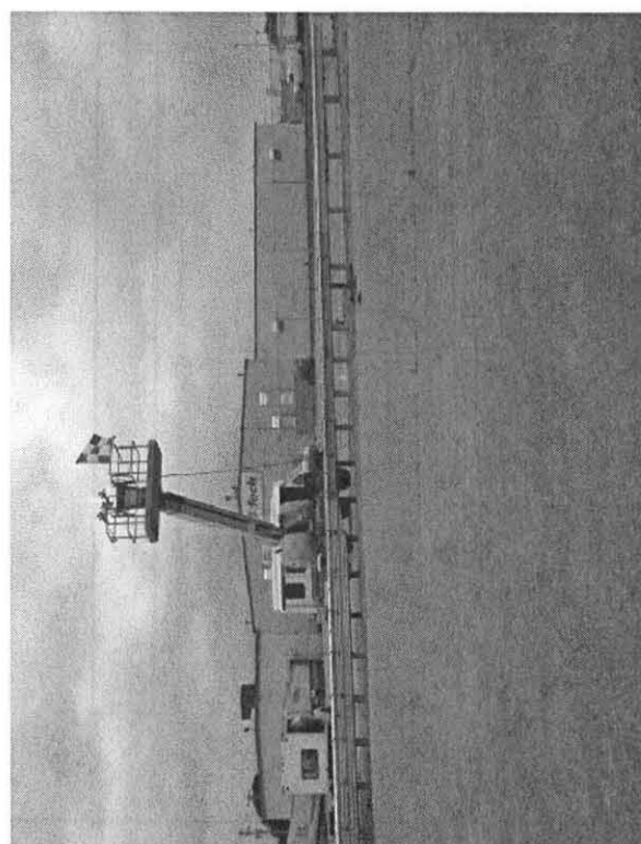
Figure 61. System and Transition Element (Design No. 2)
