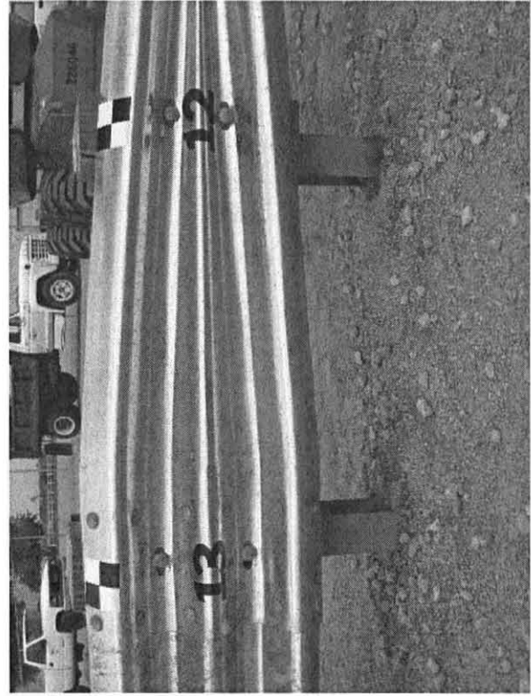
Figure 13. System and Transition Element (Design No. 1)
