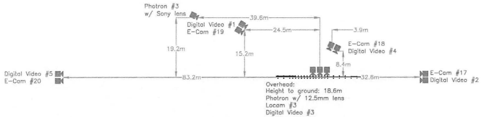
MWT-4 Camera Summary
