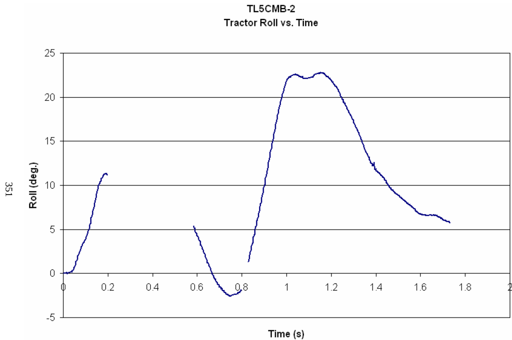
Figure F-11. Graph of Tractor Roll (Film Analysis), Test TL5CMB-2
