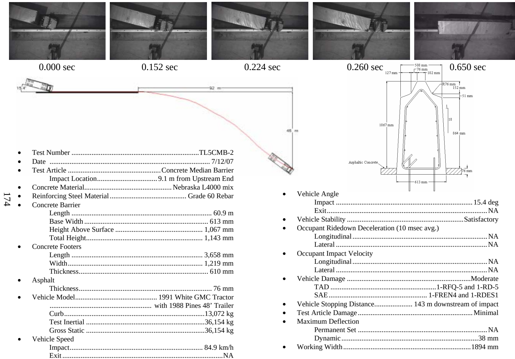
Figure 65. Summary of Test Results and Sequential Photographs, Test TL5CMB-2
