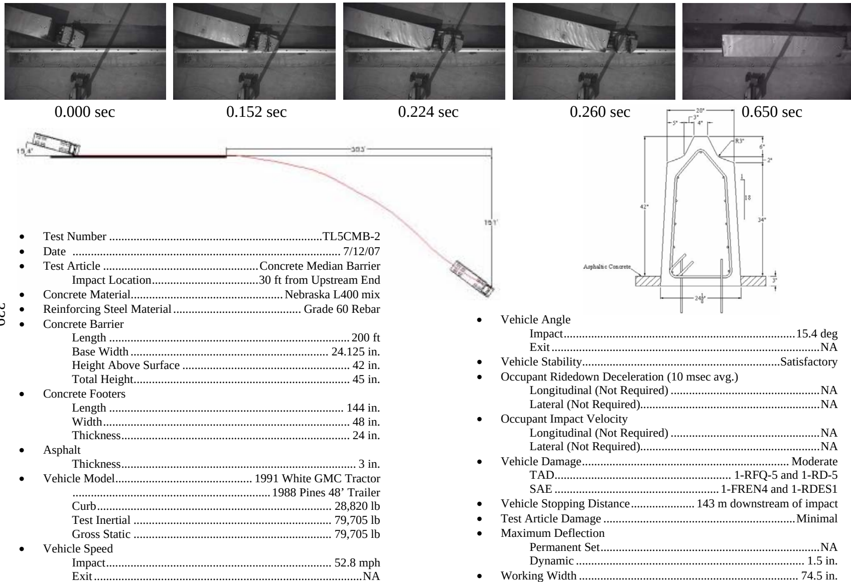
Figure E-1. Summary of Test Results and Sequential Photographs, Test TL5CMB-2
