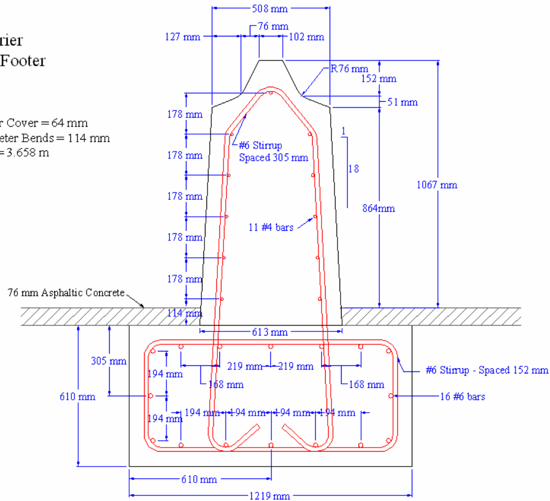
Figure 49. Footer and Barrier End Section Design
