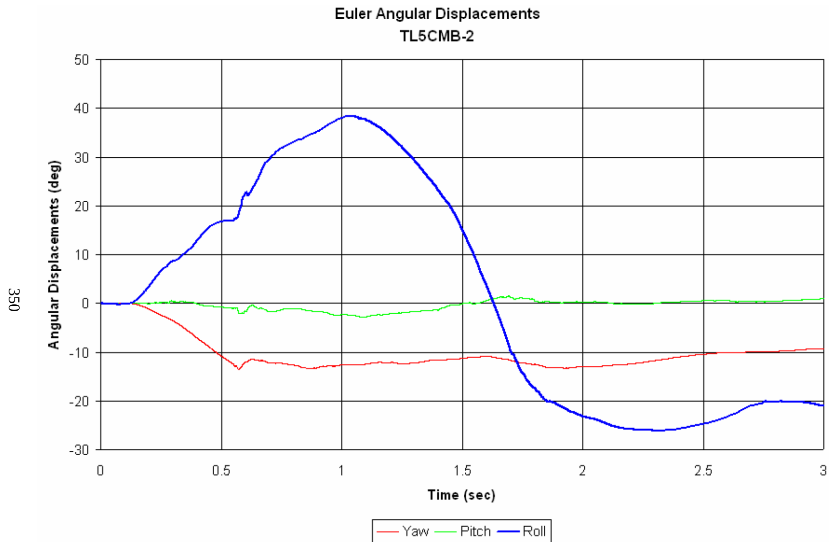
Figure F-10. Graph of Trailer Roll, Yaw, and Pitch (Gyro Data), Test TL5CMB-2
