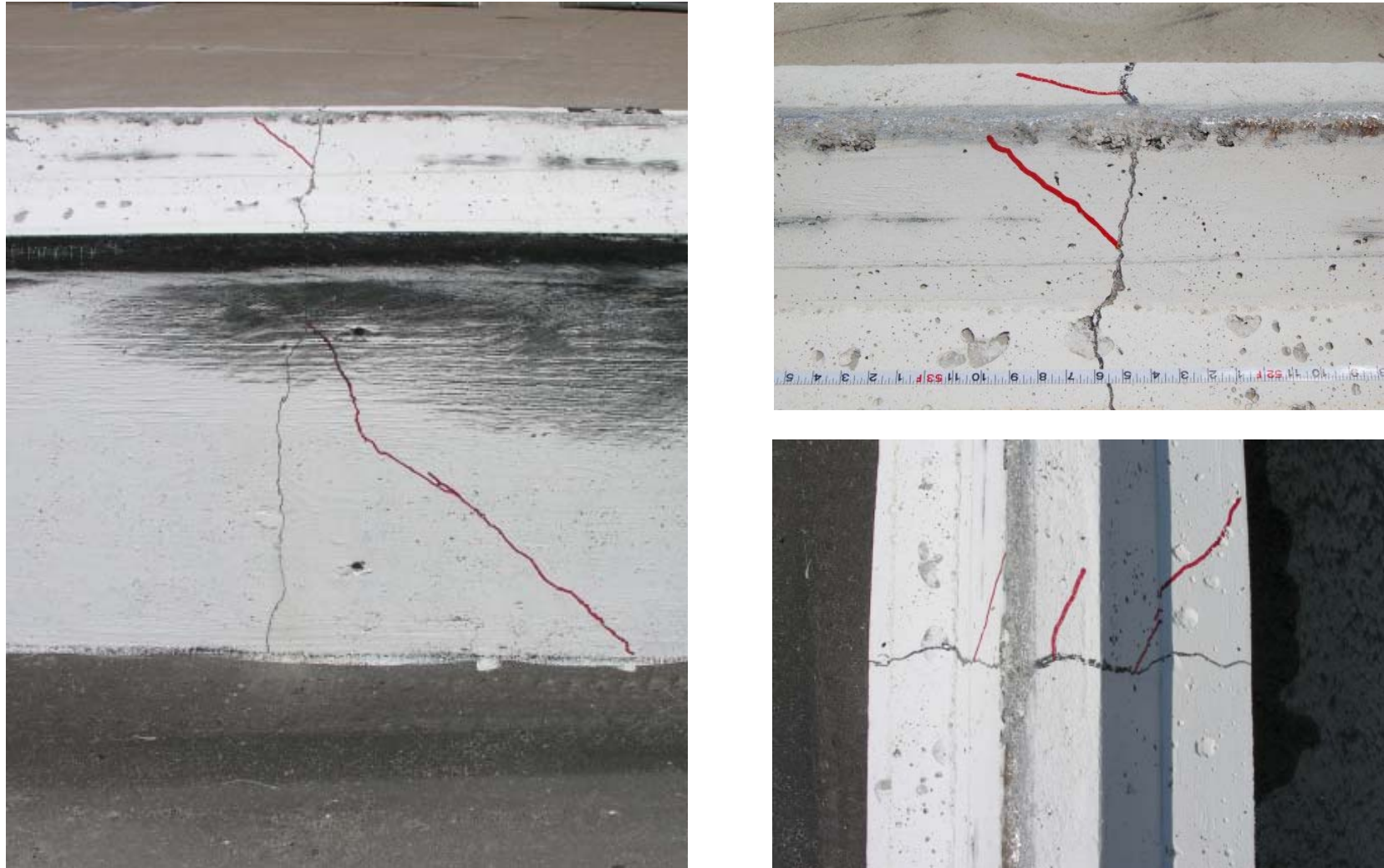
Figure 79. Barrier Cracks 15.8 m (52.5 ft) from Upstream End, Test TL5CMB-2
