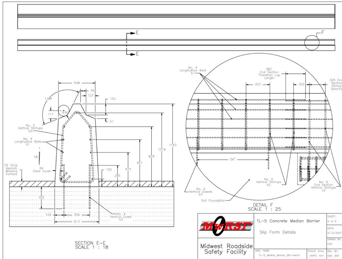
Figure 54. TL-5 Concrete Median Barrier Slipform Design Details
