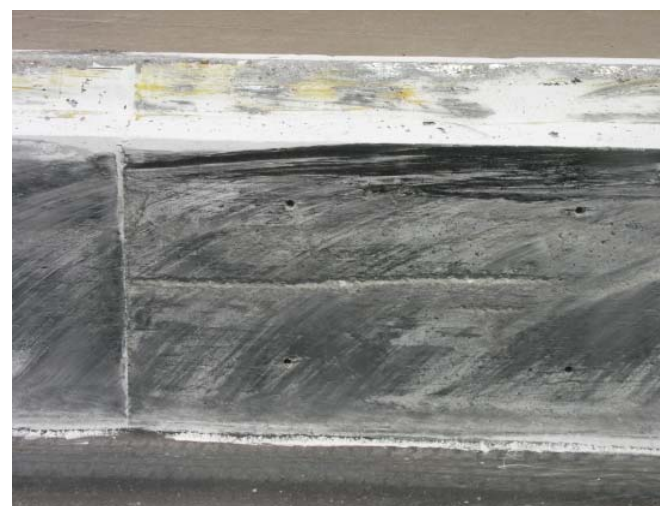
Figure 80. Barrier Damage, Gouges 9.1 - 11.0 m (30 - 36 ft) from Upstream End, Test TL5CMB-2
