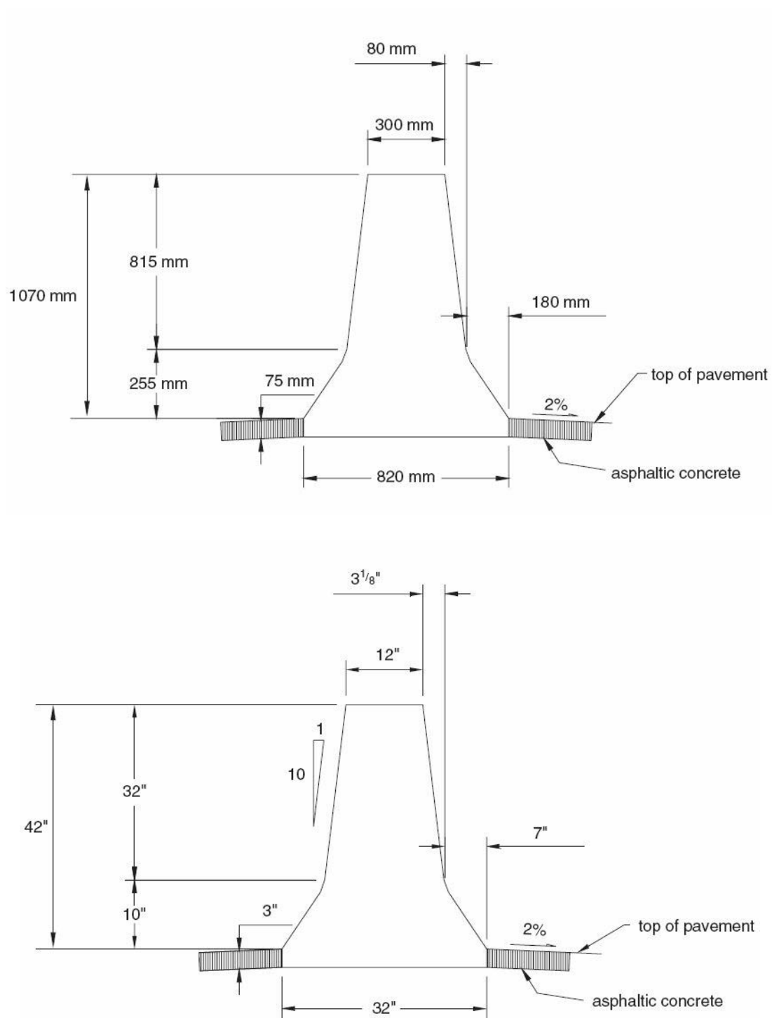
Figure 96. Non-Reinforced Concrete Tall Wall Safety Shaped Barrier [18, 20]
