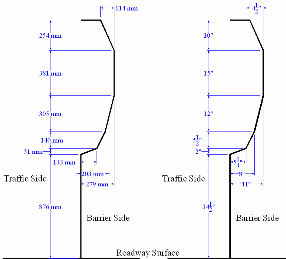
Figure 32. Head Ejection Envelope and Dimensions
