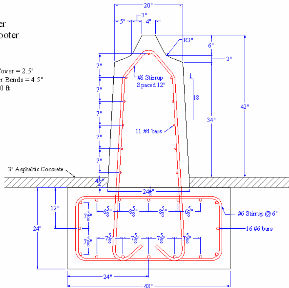
Figure 50. Footer and Barrier End Section Design (English - Units)
