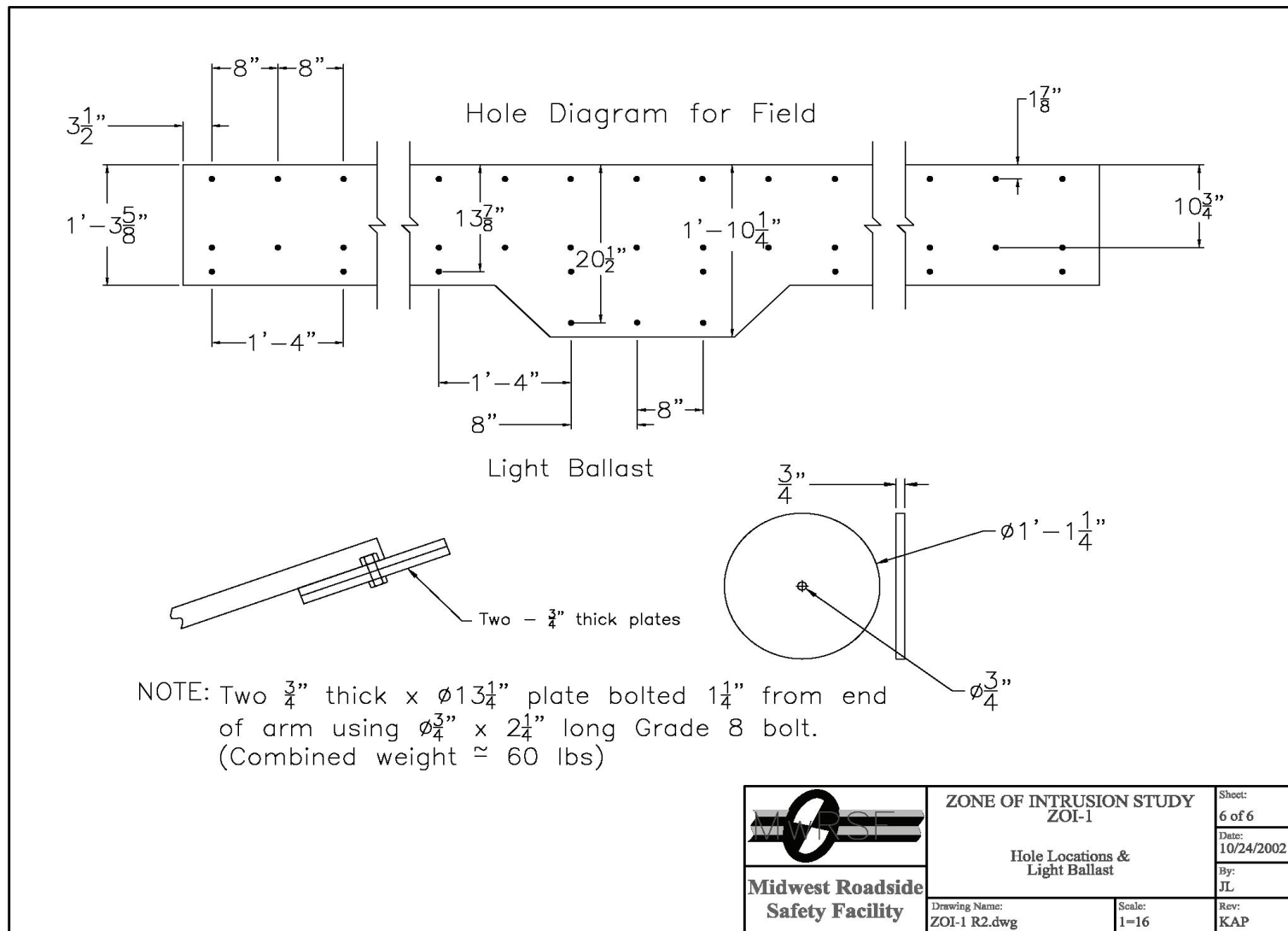
Figure C-6. Hole Locations and Light Ballast, Test No. ZOI-1 and ZOI-2 (English)
