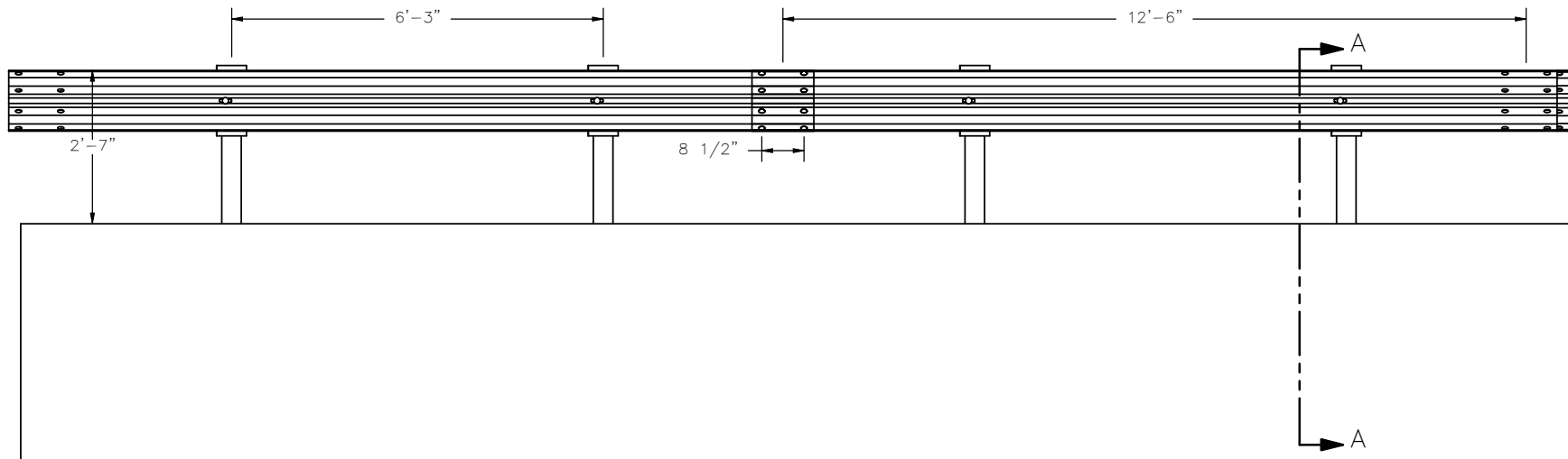
ELEVATION VIEW
