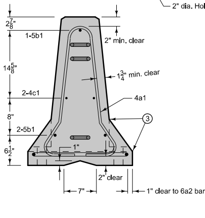
SECTION C-C Stirrup Placement
