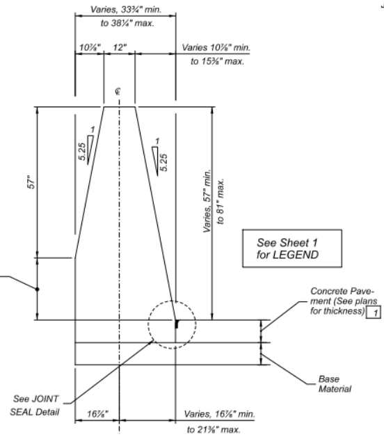
TYPE C1 (DETAIL FOR NEW CONCRETE PAVEMENT)
