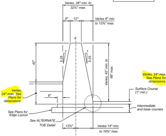
TYPE C (DETAIL FOR NEW ASPHALT PAVEMENT)
