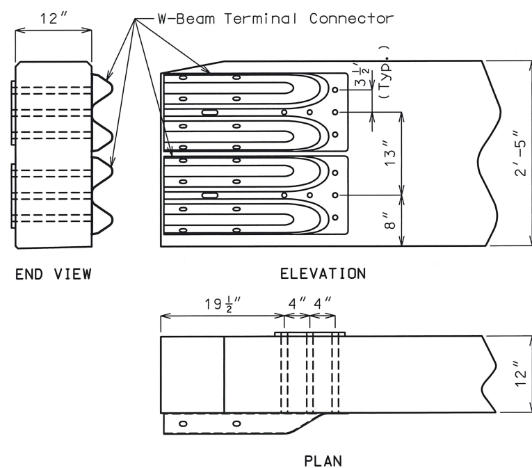
BRIDGE ANCHOR SECTION FOR 2'-5" VERTICAL BARRIER
