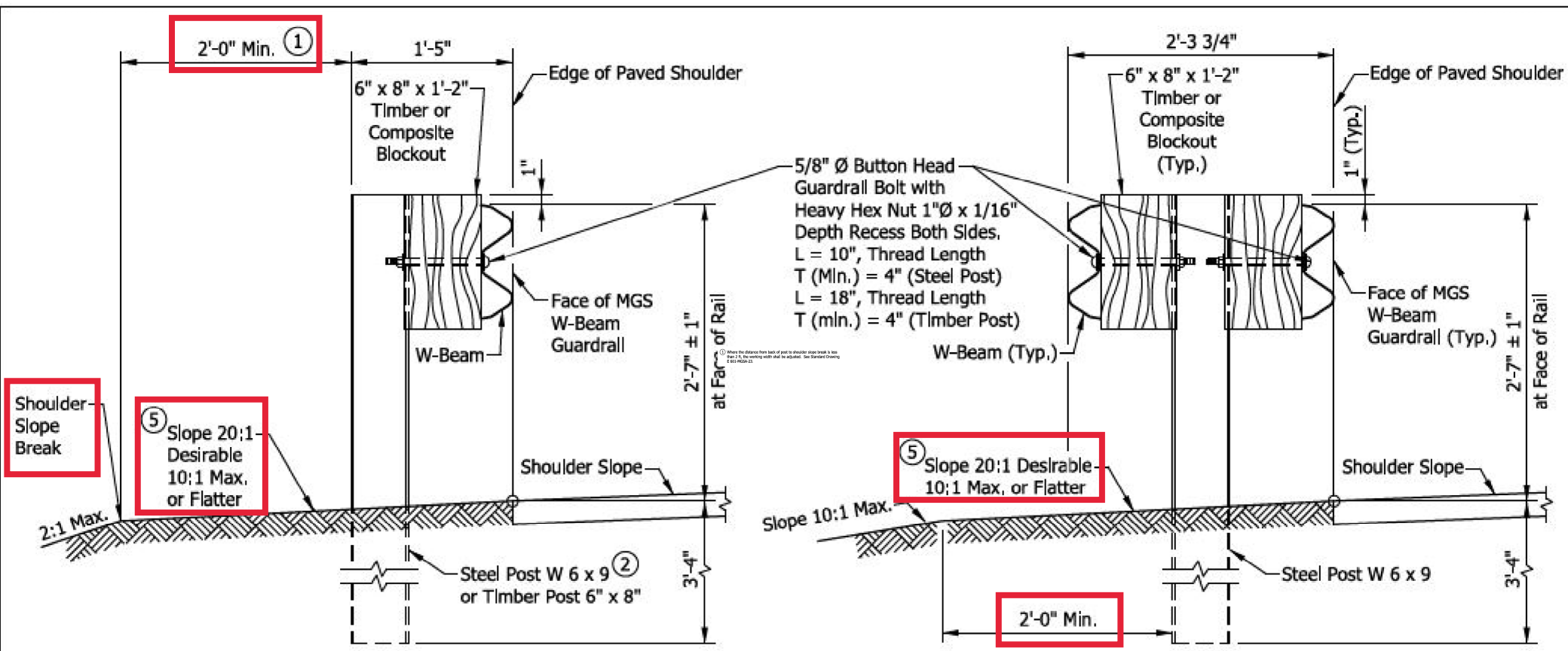
TYPICAL MGS W-BEAM INSTALLATION
