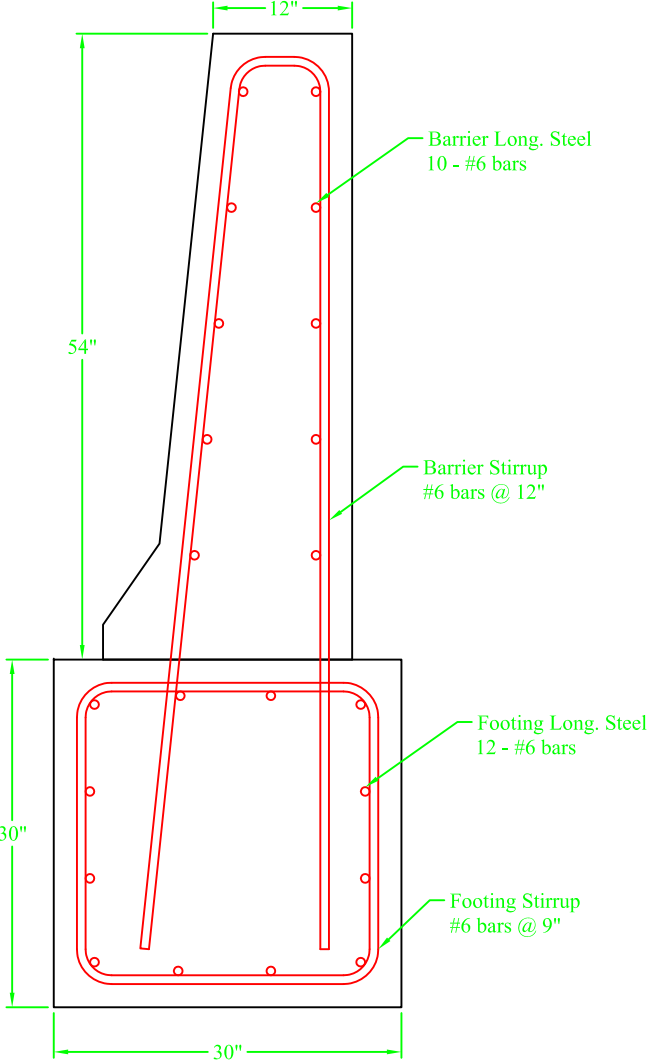
Interior Section
