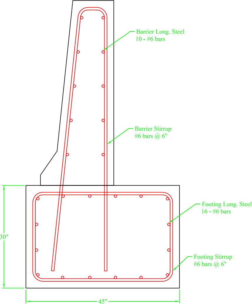
End Section - 15 ft. Minimum Length
