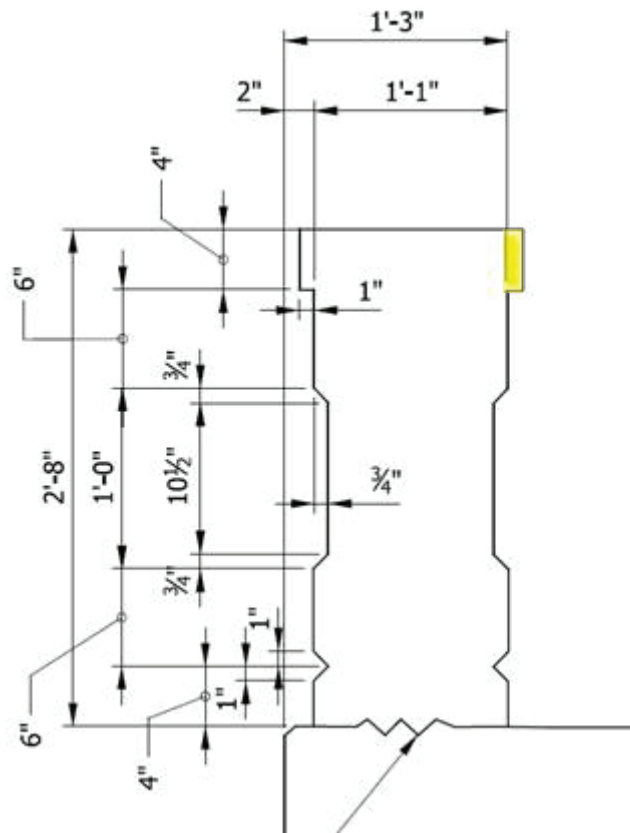
Section View
