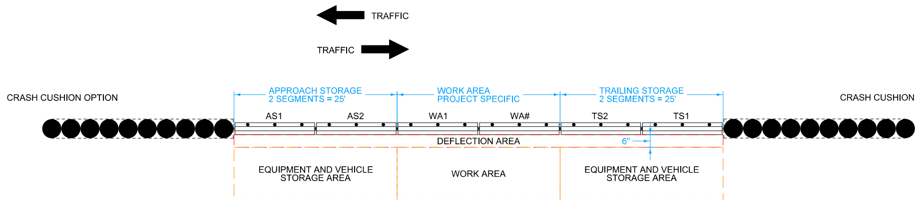
ROADSIDE APPLICATION - ANCHORED - OPPOSING TRAFFIC WITHIN CLEAR ZONE
