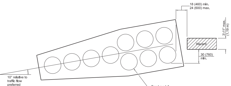
Direction of traffic flow ROADSIDE INSTALLATION (Traffic approaches on one side) (Test Level 2 array shown)
