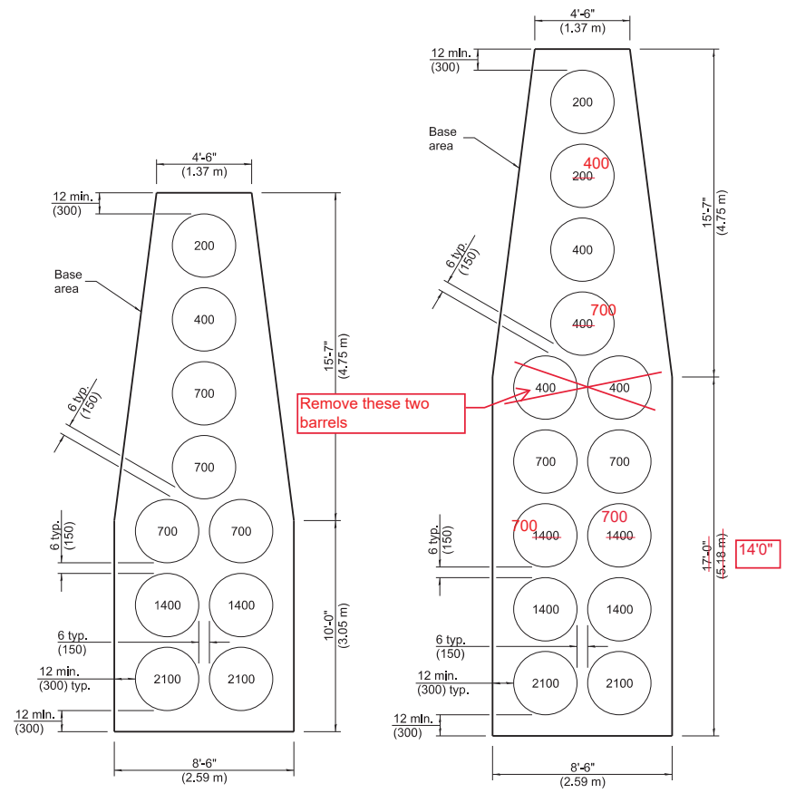
TEST LEVEL 2 ARRAY
