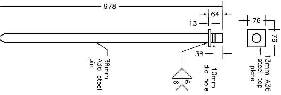
PIN ASSEMBLY FOR ASPHALT PAVEMENT
