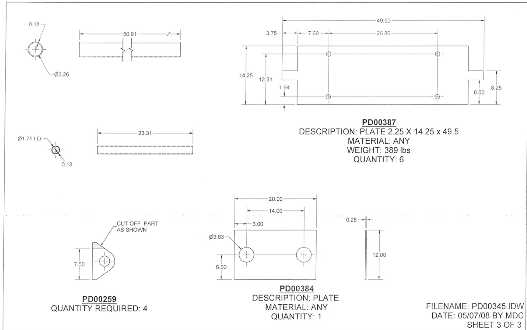
Figure 12. Pendulum Details
