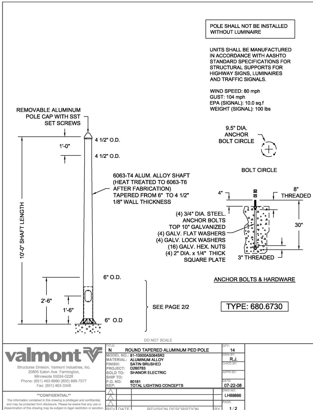
Figure 20. Aluminum Pedestrian Pole Details
