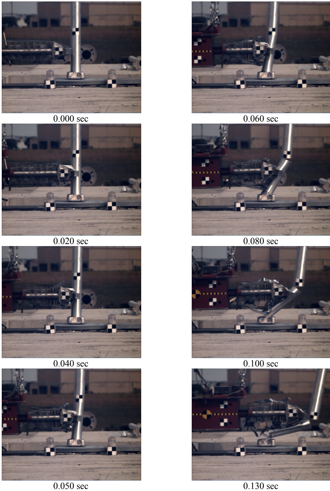
Figure 33. Sequential Photographs, Test No. NYPP-1
