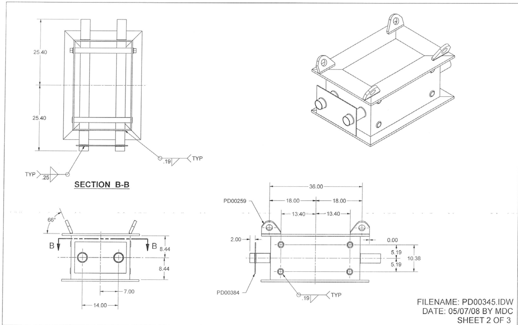
Figure 11. Pendulum Details
