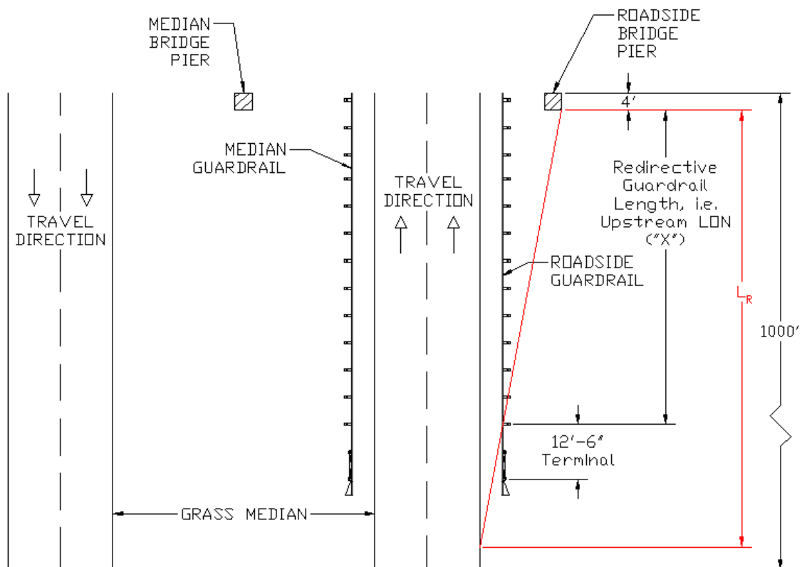
Figure 28. 1,000-ft (304.8-m) Highway Segment Plan View
