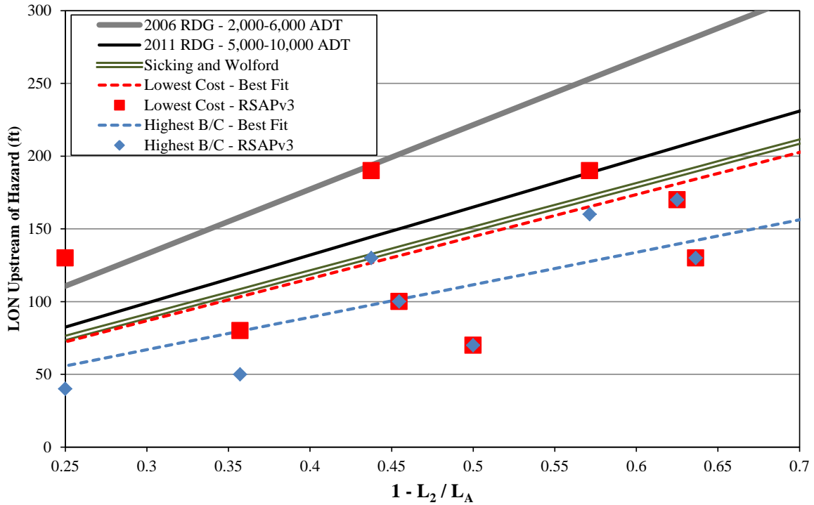
Figure 55. Recommended Guardrail Lengths for ADT < 6,000, 70 mph (113 km/h) Roadway, Left Side (Median)
