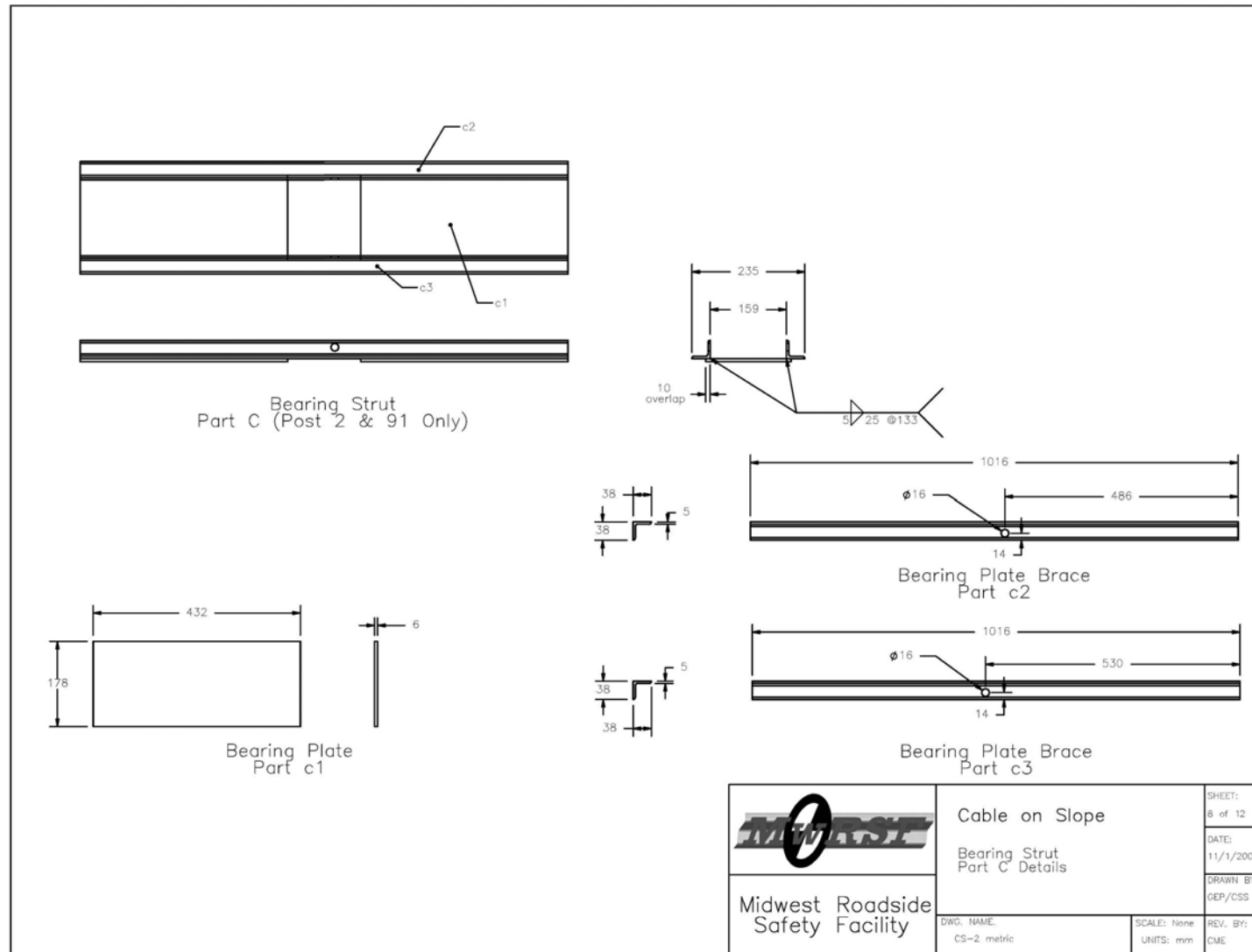
Figure 15. Bearing Strut Details
