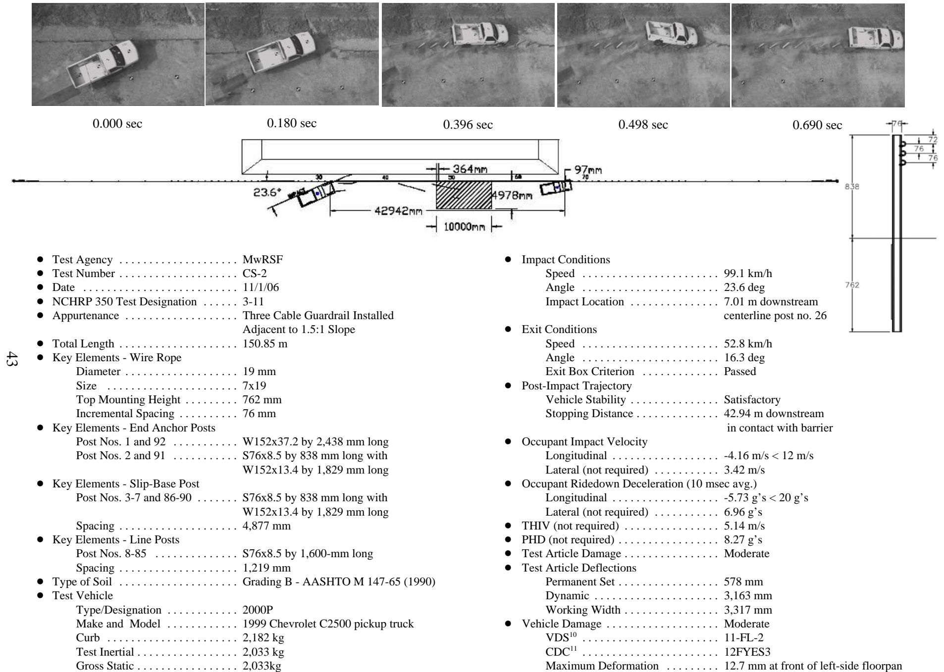
Figure 23. Summary of Test Results and Sequential Photographs, Test CS-2
