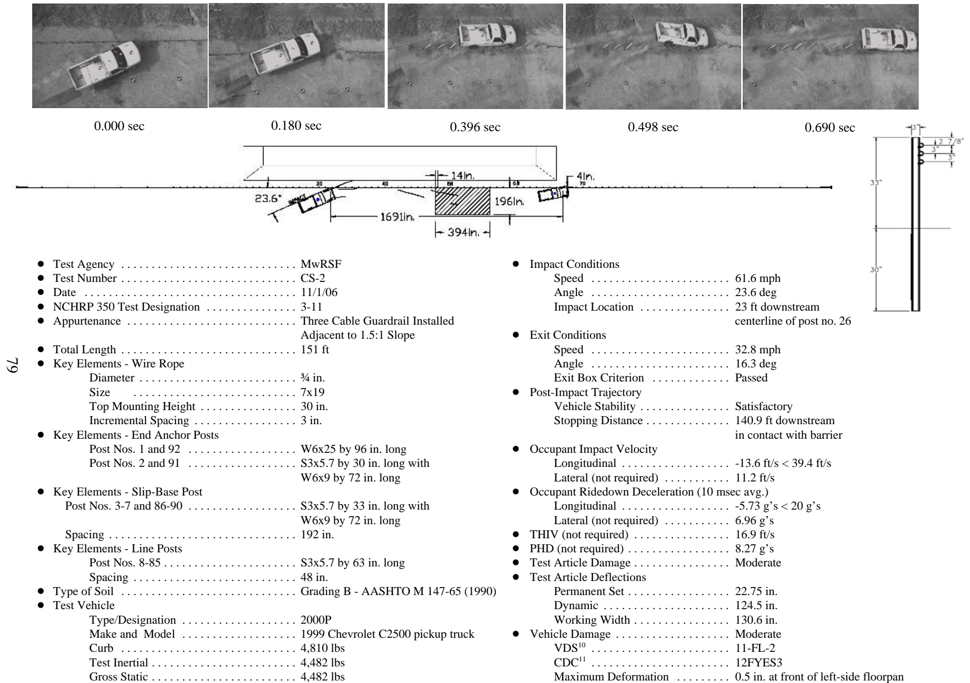
Figure B-1. Summary of Test Results and Sequential Photographs, Test CS-2
