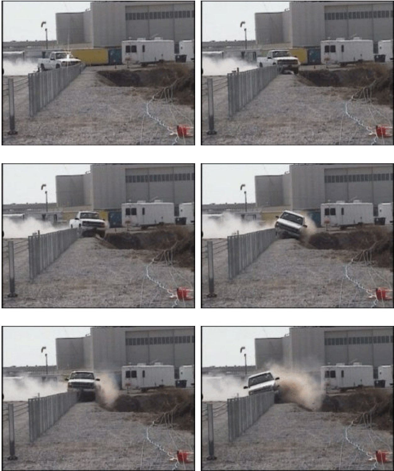
Figure 27. Documentary Photographs, Test CS-2
