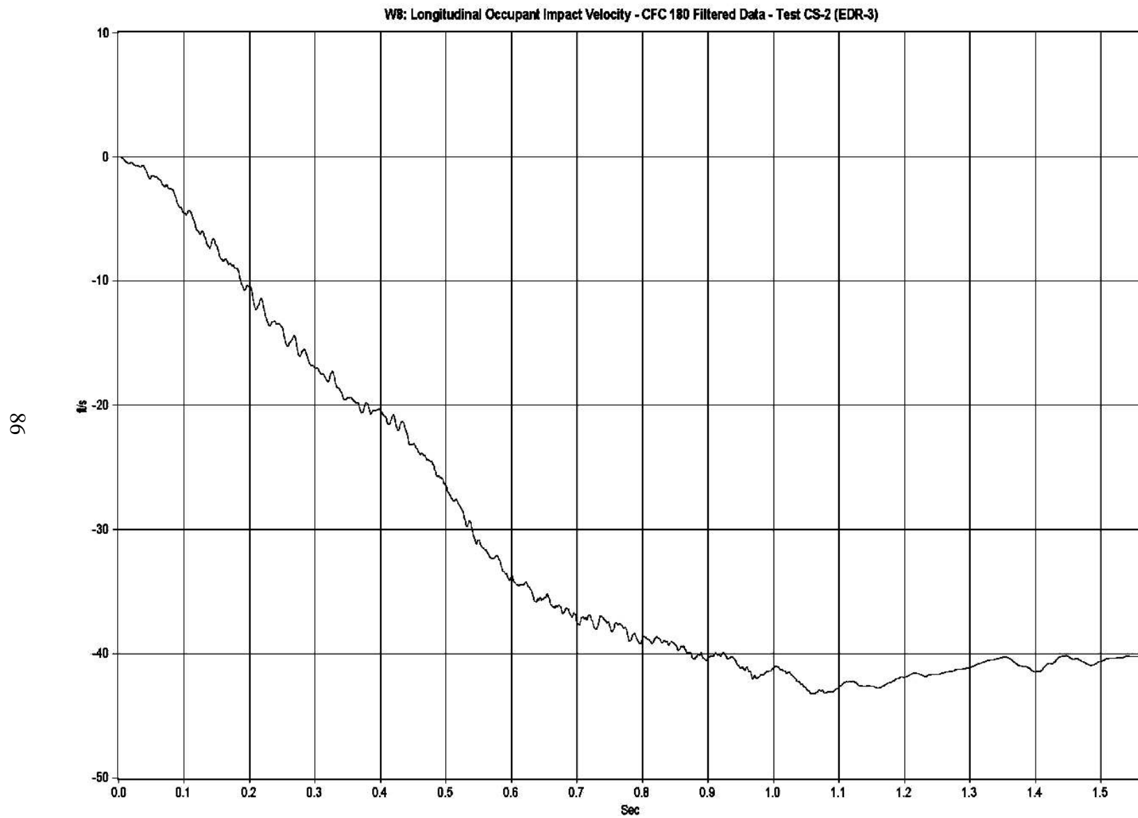
Figure D-2. Graph of Longitudinal Occupant Impact Velocity, Test CS-2
