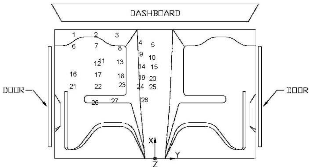
Figure C-1. Occupant Compartment Deformation Data - Set 1, Test CS-2
