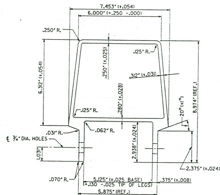
ALUMINUM CAP EXTRUSION
