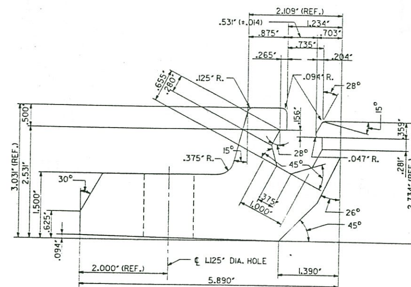
ALUMINUM TOE CLIP EXTRUSION
