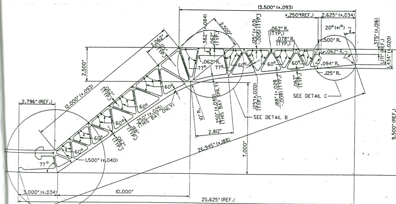
ALUMINUM PARAPET EXTRUSION
