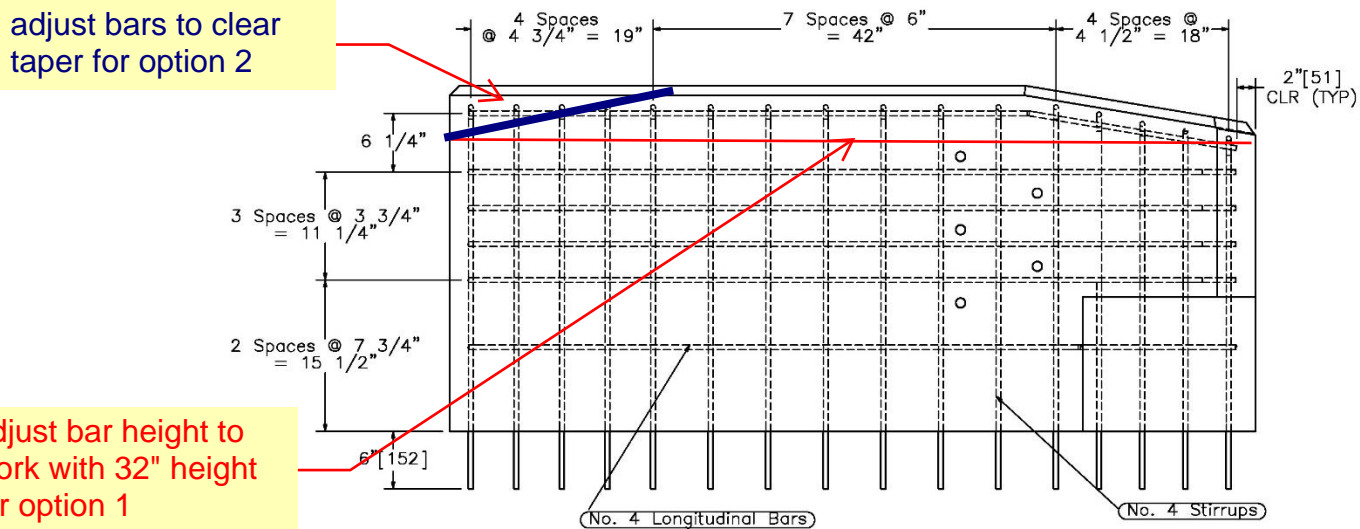
(b) Reinforcing Layout
