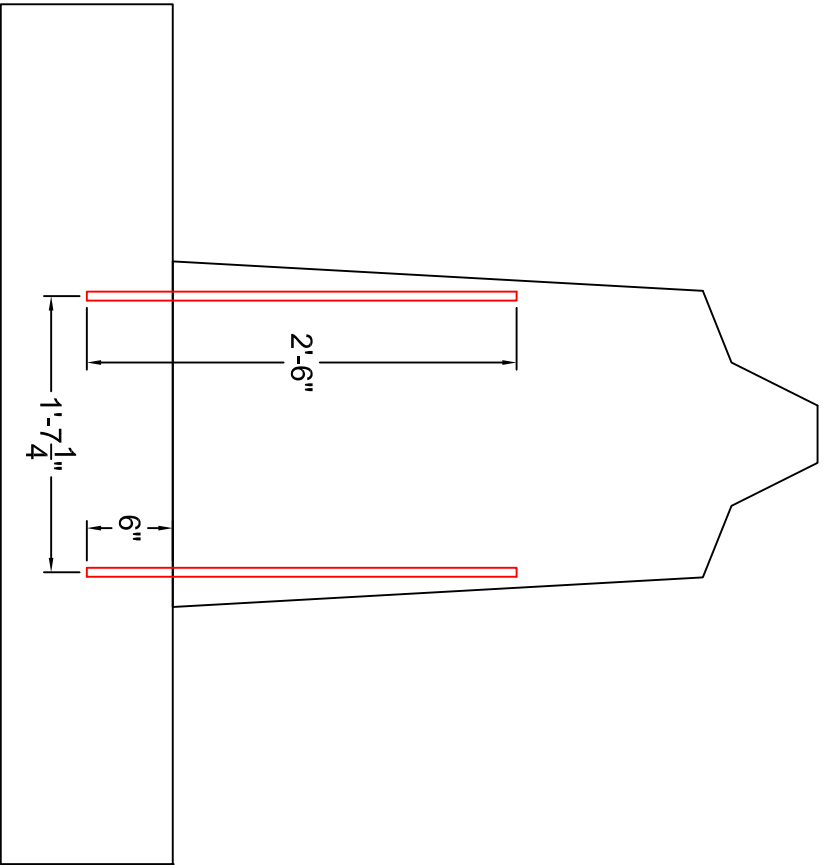
Option 2 Dowel Placement
