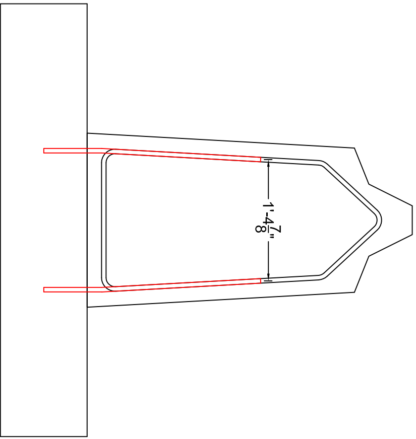
Option 2 Bend Dowels - Tie to Stirrups
