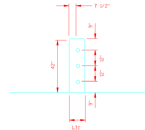
CONCRETE MASONRY ANCHORS LAYOUT
