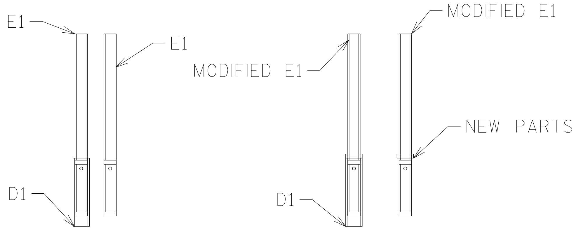
ORIGINAL MWRSF DESIGN
