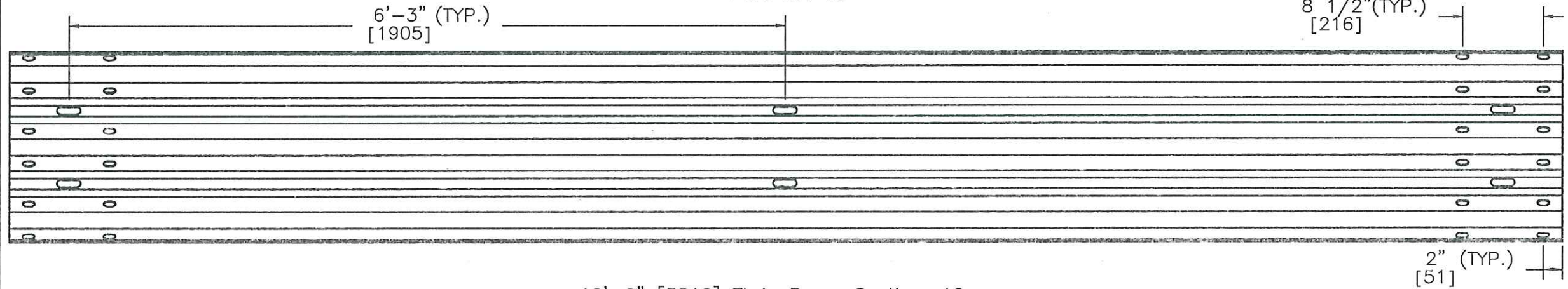
12'-6" [3810] Thrie Beam Section, 12 gauge Rail Section No. 4 Part No. b1
