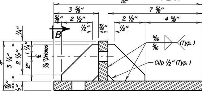
SEC. A - A
