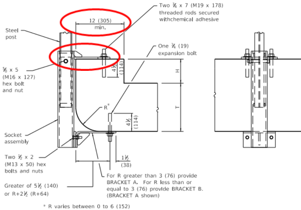
CROSS SECTION
