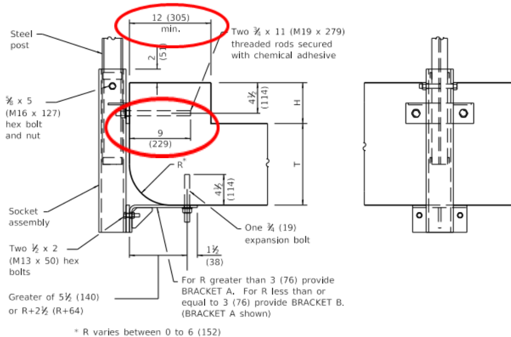
CROSS SECTION
