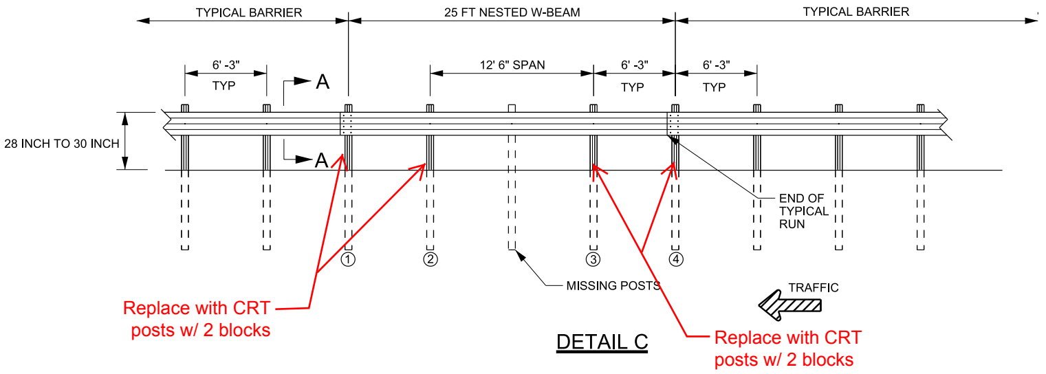
1 MISSING POST From UDOT STD DWG BA 4H1
