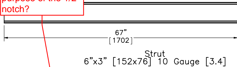
Strut and Yoke Assembly Part c3
