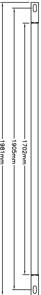
Cable Strut (Part c1)
